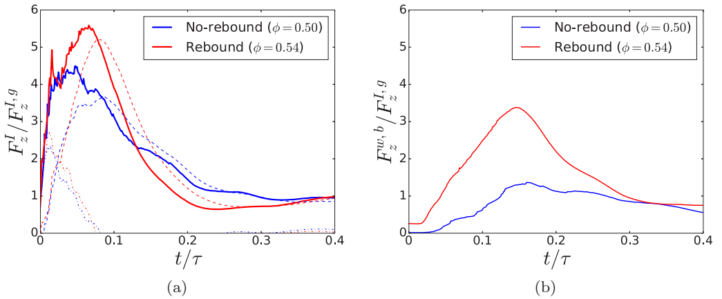
FIG. 3. Plots of the force for both rebound ( \phi = 0.54 ) and no-rebound ( \phi = 0.50 ) cases with N = 2000 . (a) Force exerted on the impactor, where the solid lines are the total force, dashed lines represent the contact contributions, and dot-dashed lines represent the hydrodynamic contributions, and (b) the total force exerted on the bottom wall. All results are obtained for \mu = 1 and u_0/u^* = 4.26 .
