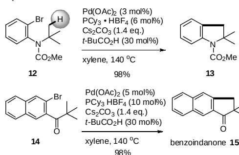
Scheme 2. Synthesis of heterocycles by Pd-catalyzed sp 3 C–H bond activation.
