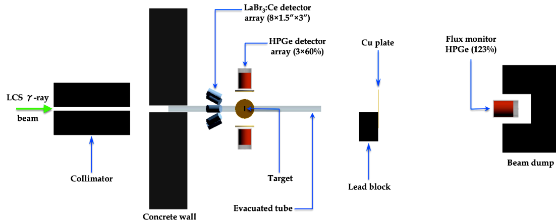
Fig. 6.13: Schematic side view of the experimental setup of the NRF measurements of the ^{238}\text{U} at the HI \gamma S facility at Duke University. The two detectors array setup was used with the 3 HPGe and the 8 LaBr 3 :Ce detectors.
