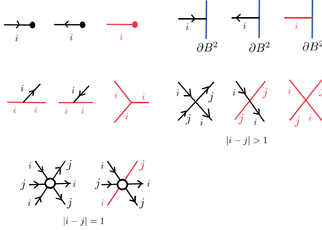
Figure 2: Vertices of a BMW chart.
