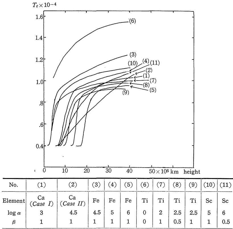
Fig. 13. 31 Cygni: T_e versus height.
