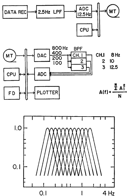
Fig. 3 Analytical system and frequency responses of band-pass filters.
