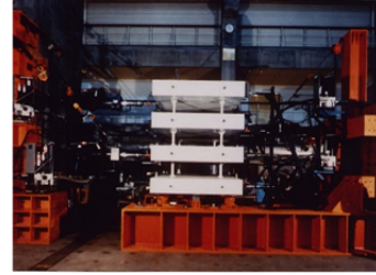
On-Line Test for Overall Structure
