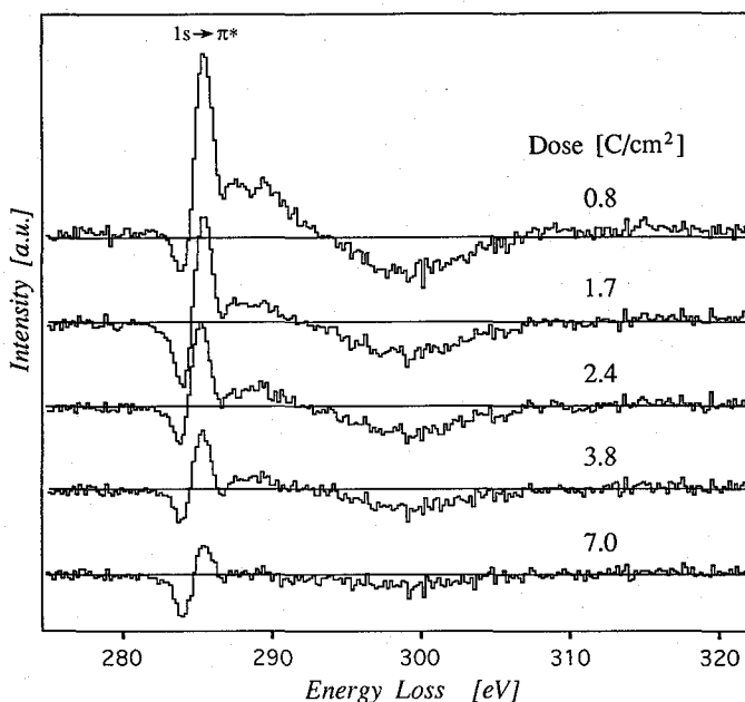
Figure 5 : Difference spectra obtained by subtracting the spectrum observed after 20 C/cm 2 from that at several stages during an electron irradiation.
