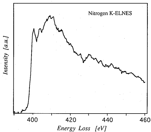
Figure 6 : Nitrogen K-edge spectrum of poly GeO-Pc measured after total dose of 0.8 \text{ C/cm}^2 . Little change in the ELNES was observed at further irradiation dose.
