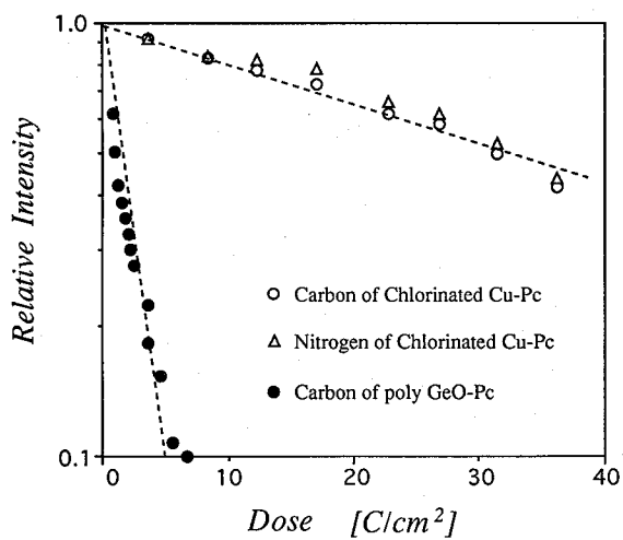
Figure 7 : Dose-response curves obtained by fading of the 1s \rightarrow \pi^* transition peak in carbon and nitrogen K-edge of poly GeO-Pc and chlorin-
