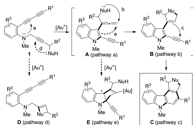
Scheme 2. Our Concept: Fused Carbazole Synthesis via Rearrangement of a Propargyl Group
