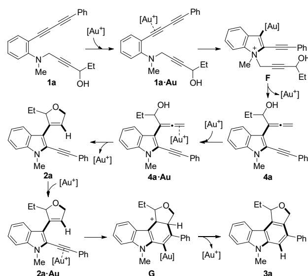
Scheme 5. Postulated Reaction Mechanism
