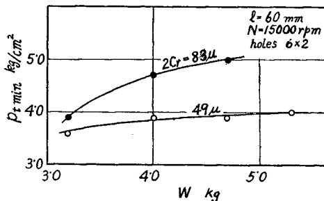
Fig. 11. Relation between suitable pressure p_{t\min} and bearing load W
