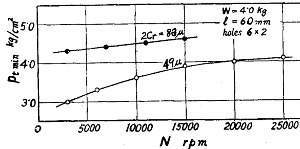
Fig. 12. Relation between suitable pressure p_{t\min} and rotational speed N ( l=60\text{mm} )
