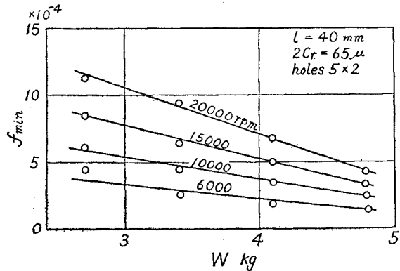
Fig. 7. Relation between f_{\min} and bearing load W
