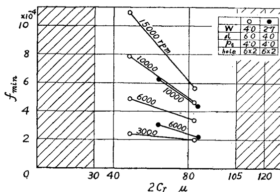
Fig. 8. Relation between f_{\min} and diametral clearance 2c_r
