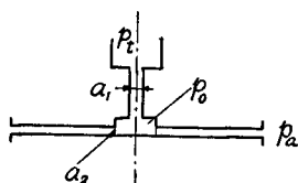
Fig. 1. A path of air-flow at an air-feeder hole
