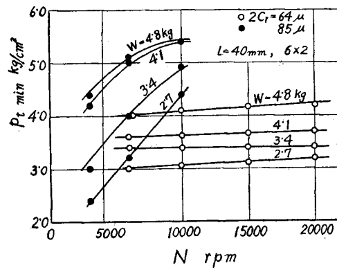
Fig. 13. Relation between suitable pressure p_{t\min} and rotational speed N ( l=40\text{mm} )
