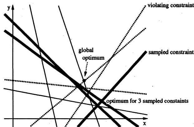
Figure 2.4. A randomized algorithm for linear programming
