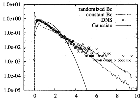
Figure 7: 絶対値の PDF, n = 16 (シェルモデル), j = 7 (DNS).
