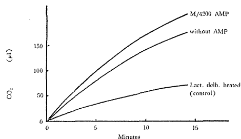
Evolution of CO 2 from pyruvate Fig. 3. Effect of AMP on the formation of CoC from V B 1 .
