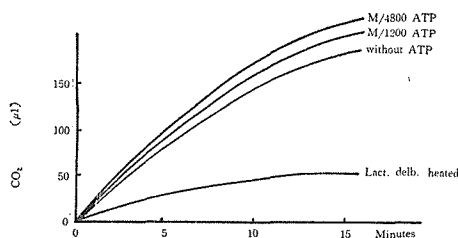
Evolution of CO 2 from pyruvate Fig. 1. Effect of ATP on the formation of CoC from V B 1 .
