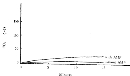
Evolution of \text{CO}_2 from pyruvate
