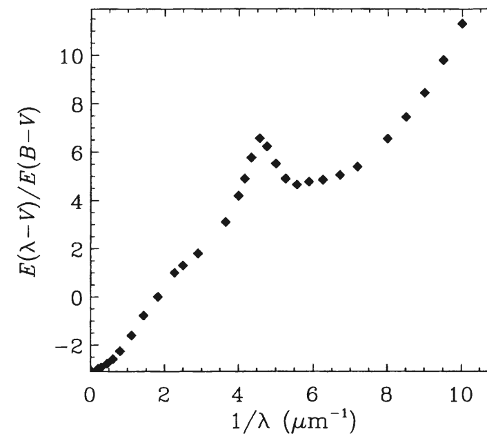
Figure 2.2: The average interstellar extinction curve ( E_{\lambda-V}/E_{B-V} versus \lambda^{-1} ). The data are taken from Table 3.1 of Whittet (1992).
