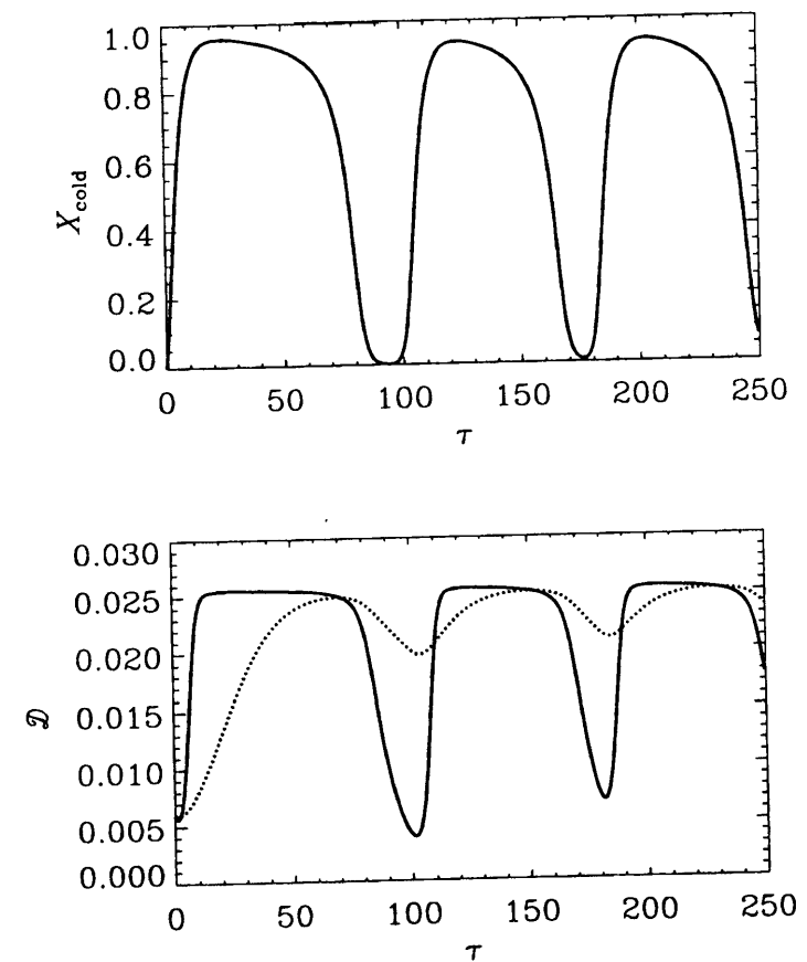
Figure 4.6: Same as Fig. 4.3, but for Model 4. The solid and dotted lines represents Models 4a and 4b, respectively. The initial condition is (X_{\text{cold}}, X_{\text{hot}}) = (0.0, 0.7) .
