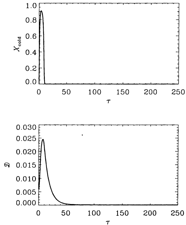
Figure 4.3: Upper panel: the time evolution of the cold-gas mass filling factor ( X_{\text{cold}} ) for Model 1. The initial condition is (X_{\text{cold}}, X_{\text{hot}}) = (0.0, 0.1) . The adopted values of the parameters are A = 1.2 , B = 3.0 , and c_*\tau_{\text{SF}} = 100 . The timestep is normalized by c^{-1} \simeq 3 \times 10^7 yr. Lower panel: the time evolution of the dust-to-gas ratio ( \mathcal{D} ).
