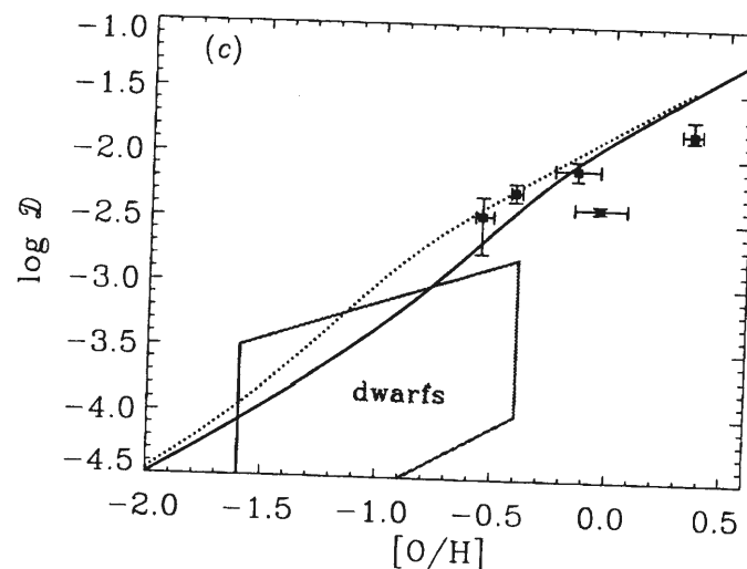
Figure 3.1: Continued. (c) Same as (a), but for various x (the slope of IMF). Here, f_{\text{in},\text{O}} = 0.1 , \beta_{\text{grow}} = 10 , and \beta_{\text{SN}} = 5 are assumed. The solid and dotted lines represent the cases of x = 2.35 and 2.7 , respectively.
