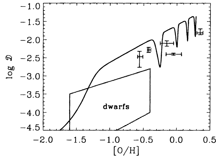
Figure 4.8: Relation between dust-to-gas ratio and oxygen abundance for the same model as Fig. 4.7. The same data as Figs. 3.1a–c are adopted.
