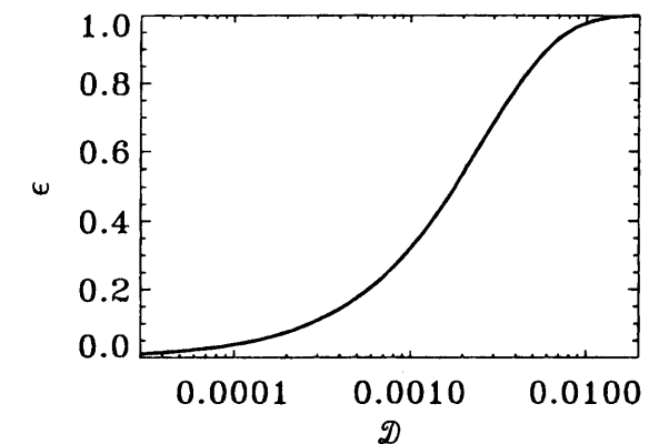
Figure 5.2: Fraction of the nonionizing photons absorbed by dust, \epsilon , as a function of the dust-to-gas ratio, \mathcal{D} .
