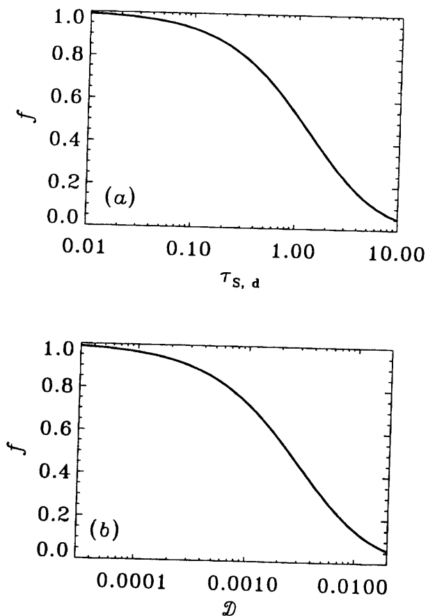
Figure 5.1: (a) Fraction of the ionizing photons absorbed by hydrogen, f , as a function of \tau_{S,d} (optical depth of dust for the nonionizing photons over a distance equal to the Strömgren radius). (b) Fraction of the ionizing photons absorbed by hydrogen, f , as a function of the dust-to-gas ratio, \mathcal{D} .
