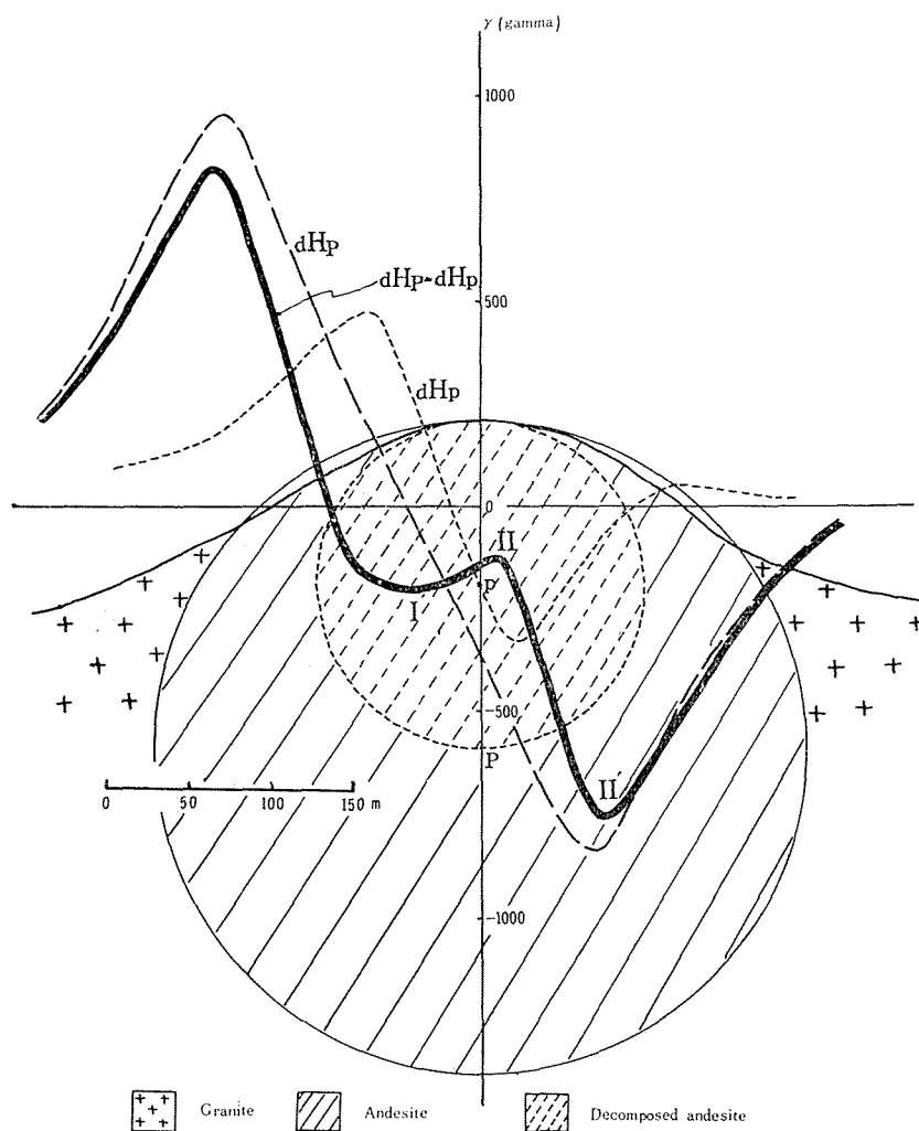
Fig. 10. Profiles of the calculated horizontal anomaly under assumption of modified model at the top of tholoid, whose radius is 100 m and intensity of magnetization 3/5 of the uneroded part, where dHp shows the anomaly due to large sphere P , dHp the anomaly due to small sphere p , and (dHp-dHp) the resultant.
