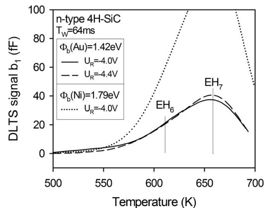
FIG. 2. DLTS spectra taken on the same 4H-SiC sample 2 with a Au Schottky barrier at reverse biases U_R=-4 V (solid curve) and U_R=-4.4 V (dashed curve), respectively, and for comparison with a Ni Schottky barrier at reverse bias U_R=-4 V (dotted curve).
