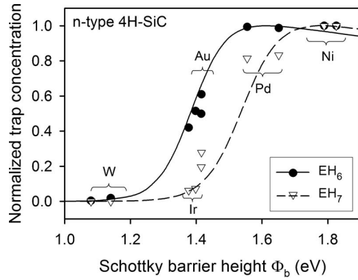
FIG. 3. Normalized trap concentration of the EH_6 and EH_7 defects (as related to the defect concentration obtained from Ni/4H-SiC Schottky contacts) as a function of the Schottky barrier height. The symbols (full circles, open triangles) are experimental data; the solid and dashed curves are theoretically calculated with Eq. (8) without using any fit parameter.
