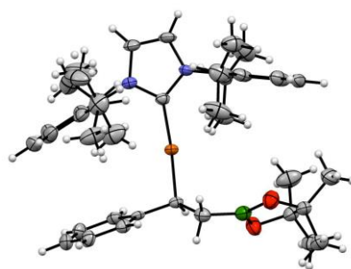
Fig. 2. Crystal structure of 2a
