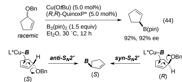
Scheme 6. A plausible reaction mechanism of the copper-catalyzed direct enantioconvergent borylation
