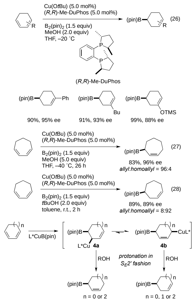
Scheme 3. A plausible reaction mechanism of the copper-catalyzed hydroboration of 1,3-dienes
