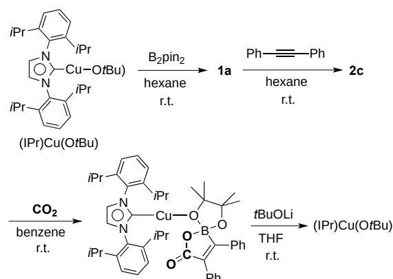
Scheme 9. Stoichiometric reactions relevant to the boracarboxylation of alkynes
