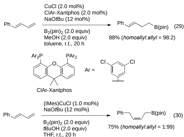
Scheme 3. A plausible reaction mechanism of the copper-catalyzed hydroboration of 1,3-dienes
