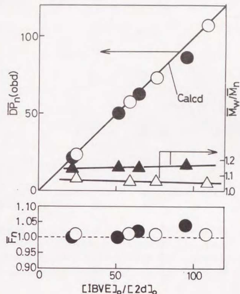
Figure 1. Effect of the initial 2d concentration ( [\mathbf{2d}]_0 ) on the \overline{DP}_n(\text{obd}) , \bar{M}_w/\bar{M}_n , and \bar{F}_n of malonate-capped polymers ( 3d ) in the IBVE polymerization by 2d /EtAlCl 2 in n -hexane at 0°C (○,△) and +60°C (●,▲): [\text{IBVE}]_0 = 0.76 \text{ M} ; [\mathbf{2d}]_0 = 7 - 35 \text{ mM} ; [\text{EtAlCl}_2]_0/[\mathbf{2d}]_0 = 1.0 (0°C) or 0.80 (+60°C); [1,4-dioxane] = 1.2 M; conversion ~ 100 %.
