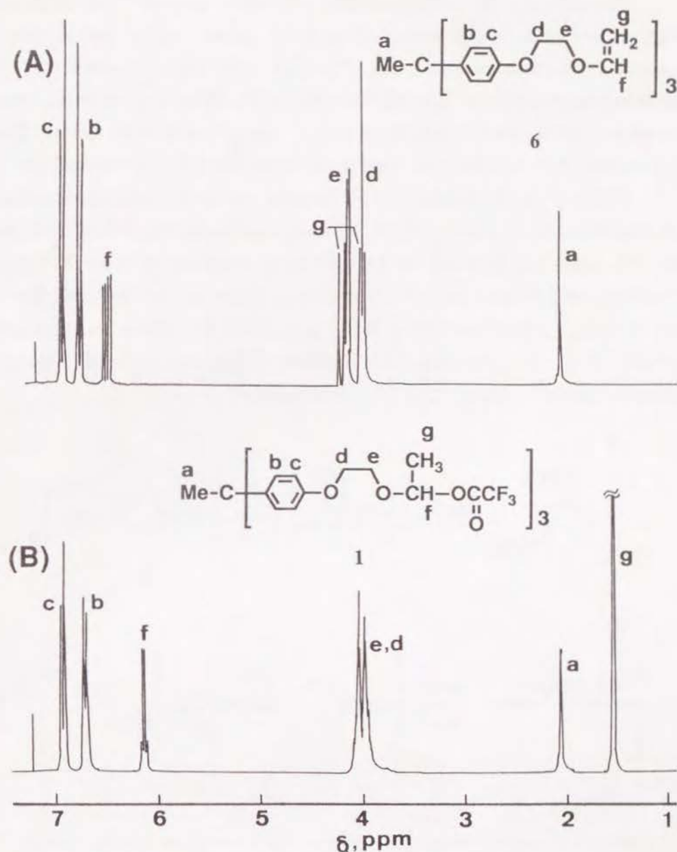
Figure 1. ^1\text{H} NMR spectra of (A) trivinyl ether 6 and (B) its trifluoroacetate form 1 .
