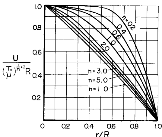
Fig. 3 Velocity distribution of pseudoplastic flow
