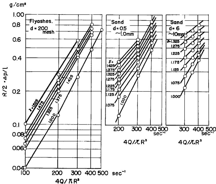
Fig. 1 Relations between R\Delta p/2l and 4Q/\pi R^3 ( D=3\text{in.} )
