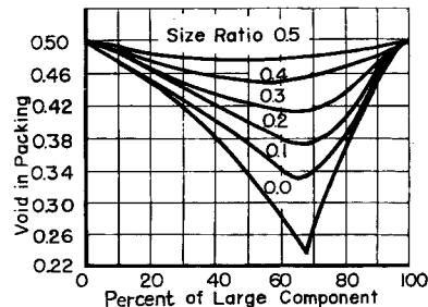
Fig. 13 Relation between void in packing and percent of large component for different size ratio 9)
