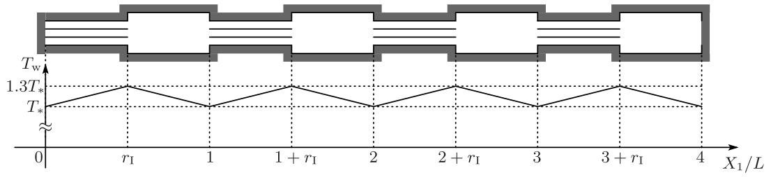
Fig. 8. Knudsen compressor and distribution of wall temperature used in the simulation in the case of N = 3 and \mathcal{N} = 4 .
