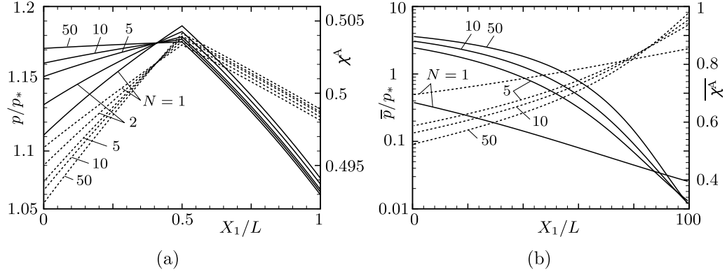
Fig. 11. Influence of the number of subdivisions in subunit I on the performance in the case of K_* = 1 , r_I = 0.5 and a_{II} = 2 . (a) Simulation of 1-unit device ( \mathcal{N} = 1 ). (b) Simulation of 100-unit device ( \mathcal{N} = 100 ). See the caption of Fig. 10.
