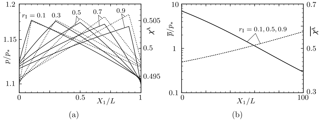
Fig. 12. Influence of the proportion of subunit I in elemental unit on the performance in the case of K_* = 1 , N = 1 and a_{II} = 2 . (a) Simulation of 1-unit device ( \mathcal{N} = 1 ). (b) Simulation of 100-unit device ( \mathcal{N} = 100 ). See the caption of Fig. 10.
