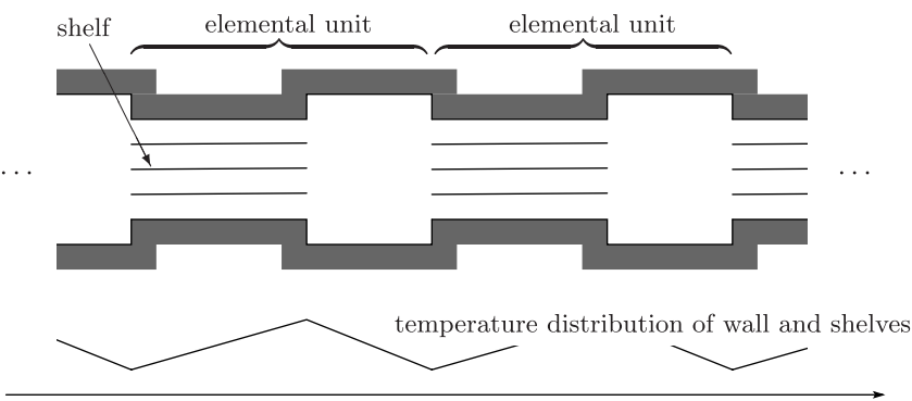
Fig. 1. Conceptual schematic of the prototype Knudsen compressor.
