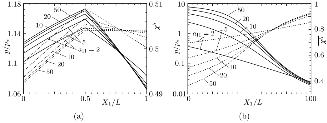
Fig. 10. Influence of the width of subunit II on the performance in the case of K_* = 1 , r_I = 0.5 and N = 1 . (a) Simulation of 1-unit device ( \mathcal{N} = 1 ). (b) Simulation of 100-unit device ( \mathcal{N} = 100 ). The solid lines indicate the profiles of the concentration of species A, while the dashed lines those of the pressure of the mixture. In (b), the pressure and concentration averaged in each unit, \bar{p} and \bar{\chi}^A , are shown at the middle point of each unit.
