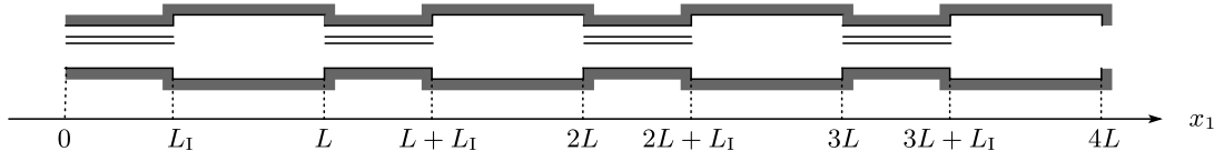
(b) A series of elemental units ( N = 3 and \mathcal{N} = 4 )
