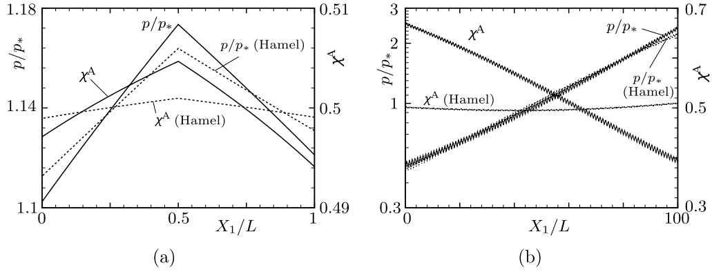
Fig. 9. Performance of the Knudsen compressor as a gas separator in the case of K_* = 1 , r_I = 0.5 , N = 1 and a_{II} = 2 . (a) Simulation of 1-unit device ( \mathcal{N} = 1 ). (b) Simulation of 100-unit device ( \mathcal{N} = 100 ). The solid lines indicate the results for the McCormack hard-sphere model, while the dashed lines with label “(Hamel)” those for the Hamel BGK-type model.
