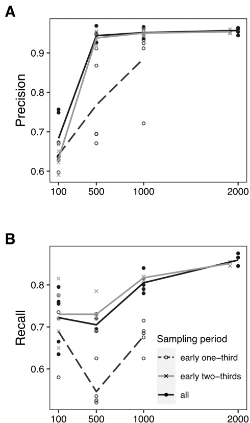
Fig. 2. Effects of dataset size and seasonal extent on model (A) precision and (B) recall. Training samples are selected from either early one-third, early two-thirds, or all of the recording period. Lines connect average values.
