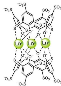
Fig. 1 Structure of \text{Ln}_3\text{TCAS}_2 complex.
