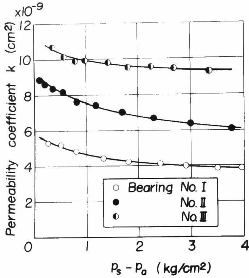
Fig. 3.2.5 Results of measurement of the permeability coefficient
