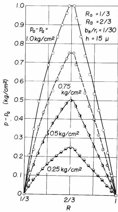
Fig. 2.4.2 Results of pressure distributions
