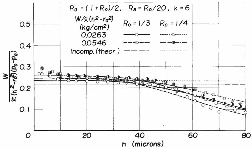
Fig. 1.4.14 Results of load capacity for various bearing parameters
