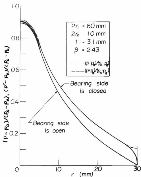
Fig. 3.2.11 Theoretical pressure distributions under open- and closed-boundary conditions
