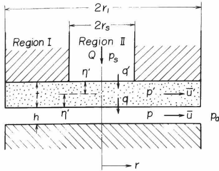
Fig. 3.2.2 Schematic diagram of the bearing
