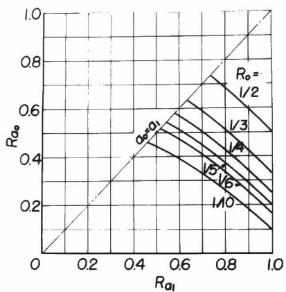
Fig. 2.3.3 Optimum positions of slit-supplies
