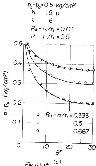
Fig. 1.3.15-1.3.18 Results of pressure distributions for various values of bearing parameters
