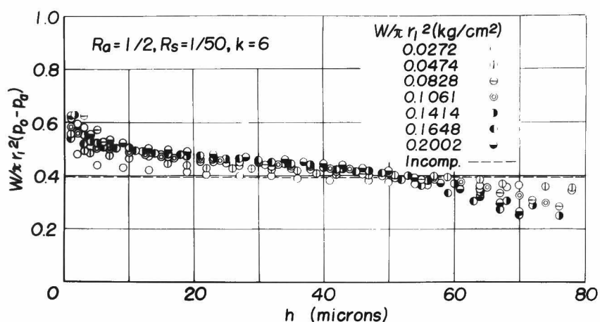
Fig. 1.3.20 Typical results of load capacity
