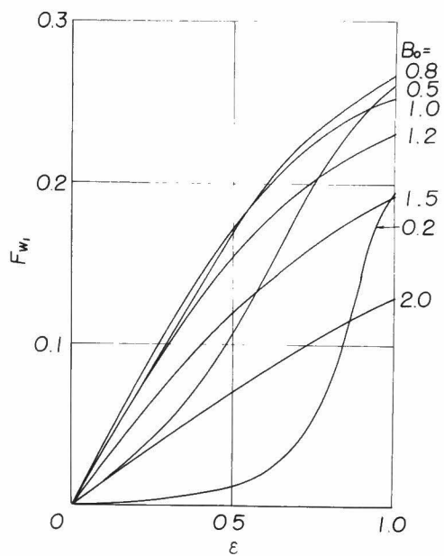
Fig. 3.4.10 Theoretical load capacity by approximation of cubic fractional expression of 1/\beta
