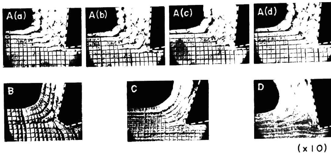
Fig. 5 Typical photographs of cutting process for lead (continuous chip formation) [Tool material, carbon tool steel; A: sharp-edged tool, (a), (b), (c), and (d): periodic change of the contour of the flow region, B: flat-edged tool, C: round-nosed tool, and D: negative rake sharp-edged tool; dry]
