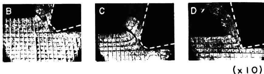
Fig. 7 Typical photographs of cutting process for Lipowitz alloy (discontinuous chip formation) [Tool material, carbon tool steel; B: flat-edged tool, C: round-nosed tool, and D: negative rake sharp-edged tool; dry]
