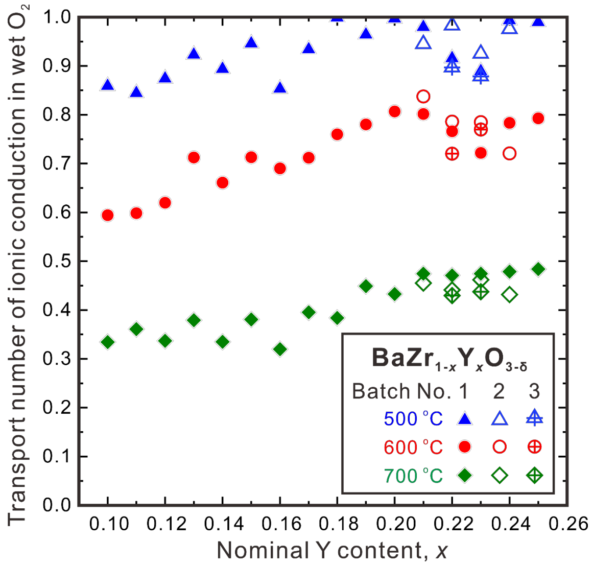
Fig. 8 Transport numbers of ionic conduction in wet O_2 ( p_{H_2O} = 0.05 atm) in the nominally stoichiometric BaZrO_3 doped with various amount of Y. Additional batches of samples of BaZr_{1-x}Y_xO_{3-\delta} ( x = 0.21, 0.22, 0.23, 0.24 ) were prepared and tested to check the reproducibility.
