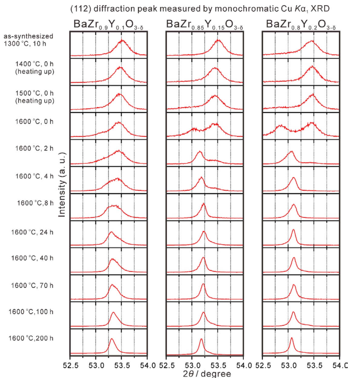
Fig. 4 Change in shape of (112) diffraction peaks collected with monochromatic Cu K\alpha_1 radiation of \text{BaZr}_{0.9}\text{Y}_{0.1}\text{O}_{3-\delta} , \text{BaZr}_{0.85}\text{Y}_{0.15}\text{O}_{3-\delta} and \text{BaZr}_{0.8}\text{Y}_{0.2}\text{O}_{3-\delta} during the heat-treatment for sintering at 1600 °C. The samples were heated up at 4.17\text{ }^\circ\text{Cmin}^{-1} from room temperature to 1000 °C, and 3.33\text{ }^\circ\text{Cmin}^{-1} from 1000 to 1600 °C. After holding at 1600 °C for up to 200 h, all the samples were quenched in ambient atmosphere.
