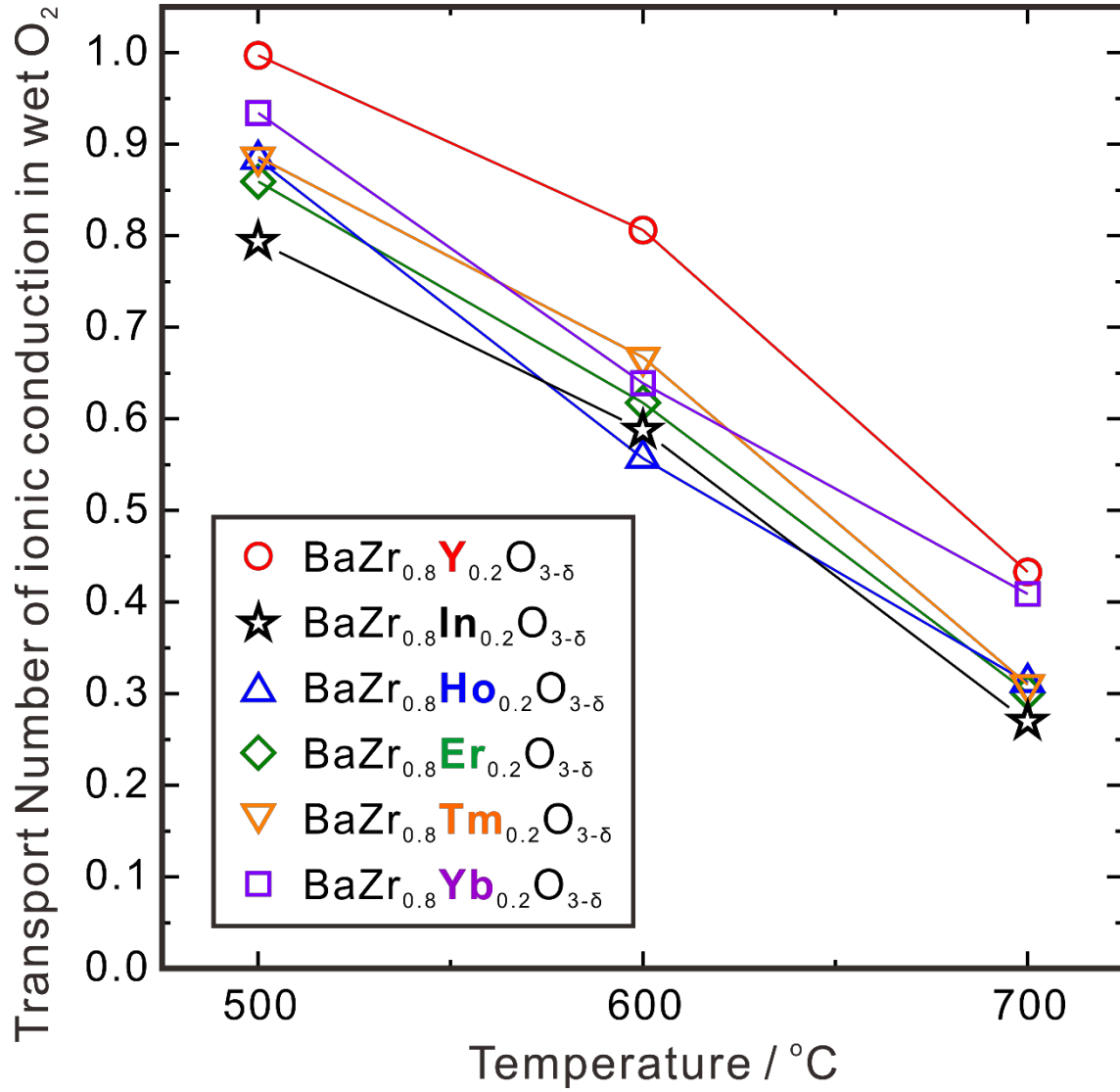
Fig. 11 Transport numbers of ionic conduction in nominally stoichiometric BaZr 0.8 M 0.2 O 3-δ (M = Y, In, Ho, Er, Tm and Yb) in wet O 2 ( p_{\text{H}_2\text{O}} = 0.05 atm). All the samples were finally heat-treated at 1600 °C in oxygen for 24 h. All samples were furnace cooled to room temperature, except BaZr 0.8 Y 0.2 O 3-δ which was quenched in ambient atmosphere.
