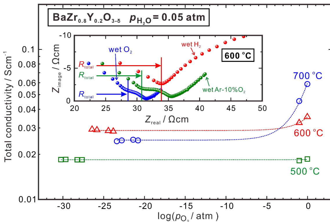
Fig. 7 Dependence of total conductivity of nominally stoichiometric BaZr 0.8 Y 0.2 O 3-δ on partial pressure of oxygen at 500, 600 and 700 °C. The impedance spectra at 600 °C in wet H 2 , Ar – 10% O 2 , and O 2 are given in the inset to show how the total resistance were determined. The sample was sintered at 1600 °C in oxygen for 24 h and quenched to room temperature. The partial pressure of water vapor in the atmosphere for collecting the impedance spectra was 0.05 atm. The composition of the sample was determined to be Ba 0.99 Zr 0.80 Y 0.20 O 3-δ by ICP-AES measurement.
