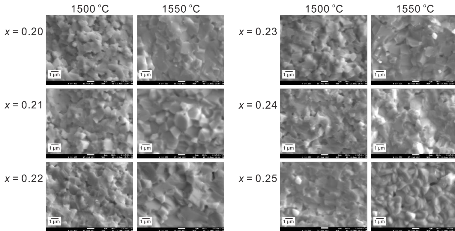
Fig. 6 EPMA second electron images of fracture cross-section area of \text{BaZr}_{1-x}\text{Y}_x\text{O}_{3-\delta} ( x = 0.20, 0.21, 0.22, 0.23, 0.24 and 0.25 ) sintered at 1500 or 1550 °C in oxygen for 24. All the samples were furnace cooled to room temperature.
