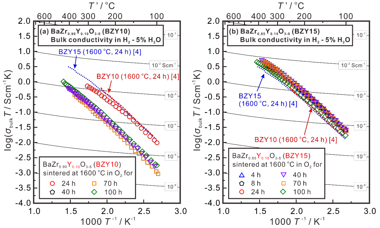
Fig. 12 Arrhenius plots of bulk conductivity in wet \text{H}_2 ( p_{\text{H}_2\text{O}} = 0.05 \text{ atm} ) of (a) \text{BaZr}_{0.9}\text{Y}_{0.1}\text{O}_{3-\delta} , and (b) \text{BaZr}_{0.85}\text{Y}_{0.15}\text{O}_{3-\delta} heat-treated at 1600^\circ\text{C} for various time for sintering. All the samples were finally quenched in ambient atmosphere.
