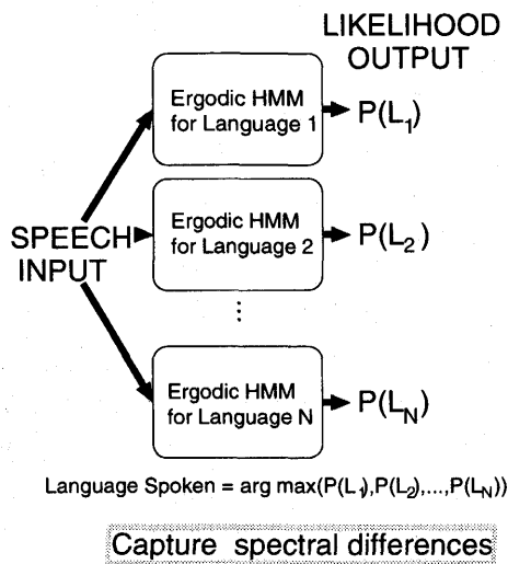
Figure 2: Ergodic HMM-based method
