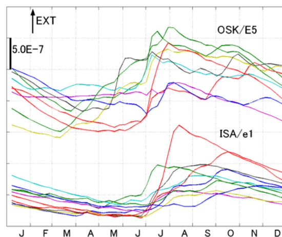
Fig. 6 Seasonal variations(SE+AR) of ground strains at OSAKAYAMA and ISA Observatory.
