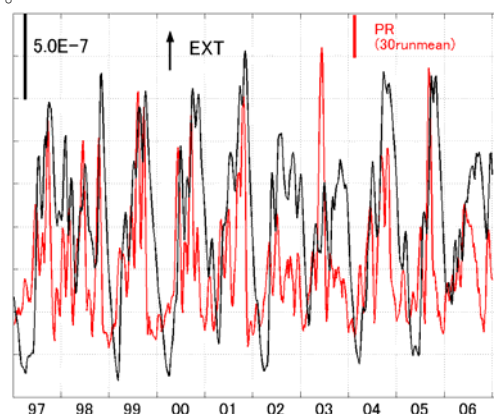
Fig. 8 Seasonal variations(SE+AR) of precipitation and ground-strains at MIYAZAKI Observatory.
