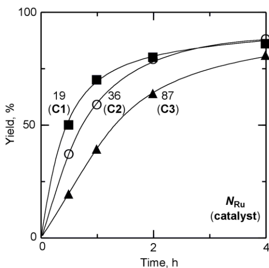
Figure 3 Effects of Ru(II) number ( N_{\text{Ru}} ) per a Ru(II)-PEG star molecule [ C1 (filled squares), C2 (open circles), C3 (filled triangles)] on the transfer hydrogenation of acetophenone ( S1 ): S1 / \text{Ru(II)} / \text{K}_2\text{CO}_3 = 10/0.010/1.0 mmol in 2-propanol (10 mL) at 100 °C.
