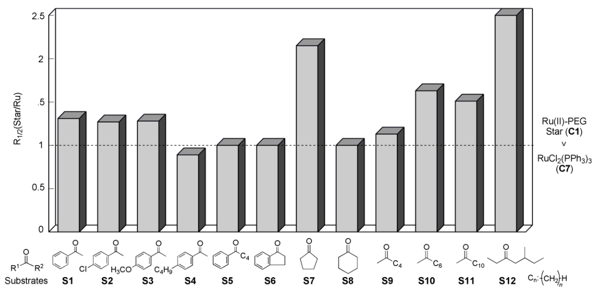
Figure 4 Catalytic activity of C1 to C7 evaluated for the relative reduction rate [ R_{1/2}(\text{Star/Ru}) ] of various substrates ( S1-S12 ). R_{1/2}(\text{Star/Ru}) = T_{1/2}(\text{C7})/T_{1/2}(\text{C1}) . T_{1/2}(\text{C7 or C1}) : half-life periods of substrates catalyzed by C7 or C1 , respectively. Conditions: substrate/Ru(II)/ K_2CO_3 = 10/0.010/1.0 mmol in 2-propanol (10 mL) at 100 °C. S6 : R_{1/2}(\text{Star/Ru}) calculated from the respective yields ( C1 , C7 = 22%) at 8 h.
