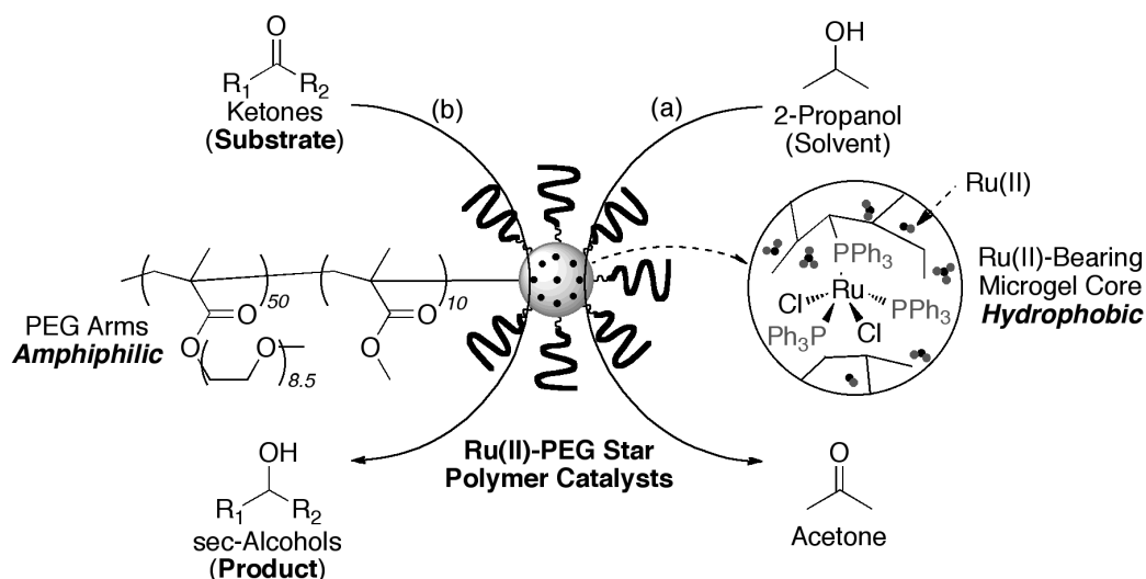
Scheme 2 Microgel-core reaction space of Ru(II)-PEG star catalysts for the transfer hydrogenation of ketones: (a) supply of a hydrogen donor (2-propanol) to core-bound Ru(II) and (b) diffusion of substrates (ketones) and products (sec-alcohols) around the microgel-core reaction space.
