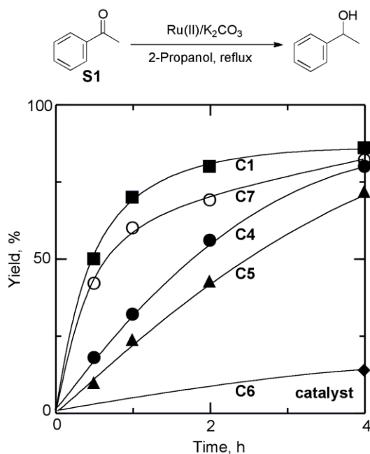
Figure 2 Transfer hydrogenation of acetophenone ( S1 ) catalyzed by various Ru(II) complexes: Ru(II)-PEG Star ( C1 : filled squares); Ru(II)-MMA Star ( C4 : filled circles); Ru(II)-Gel ( C5 : filled triangles); Ru(II)-Random ( C6 : filled diamonds); \text{RuCl}_2(\text{PPh}_3)_3 ( C7 : open circles). Conditions: S1 / \text{Ru(II)} / \text{K}_2\text{CO}_3 = 10/0.010/1.0 mmol in 2-propanol (10 mL) at 100 °C.
