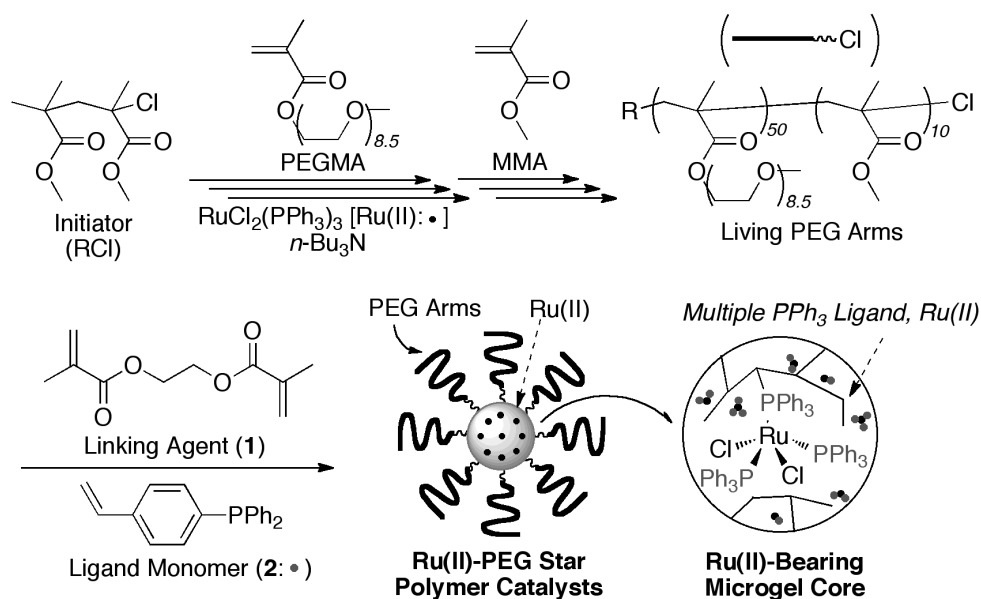
Scheme 1 One-pot synthesis of Ru(II)-PEG star polymer catalysts via Ru(II)-catalyzed living radical polymerization.
