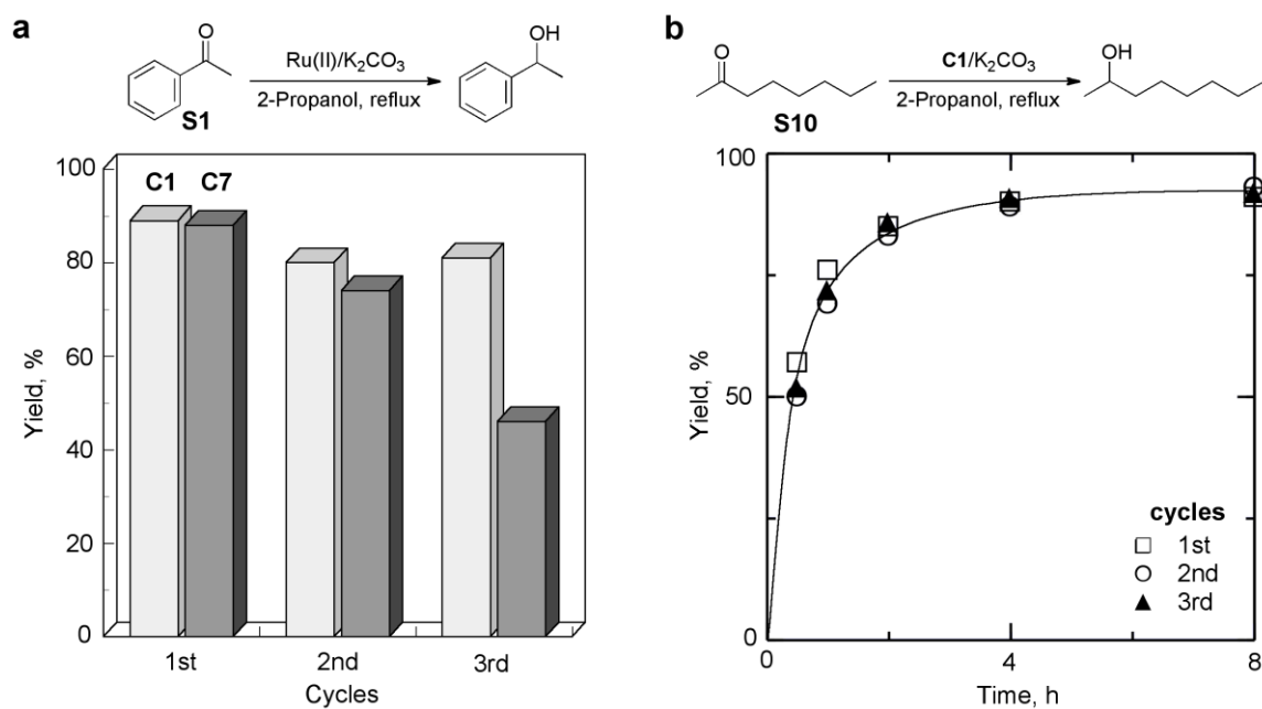
Figure 5 (a) Recycle experiments of C1 (light gray) and C7 (dark gray) for the hydrogenation of S1 . (b) Recycle experiments of C1 for the hydrogenation of S10 [cycle: 1st (open squares), 2nd (open circles), 3rd (filled triangles)]. Conditions: S1 or S10 /Ru(II)/K 2 CO 3 = 15/0.015/1.5 mmol in 2-propanol (15 mL) at 100 °C for 8 h.
