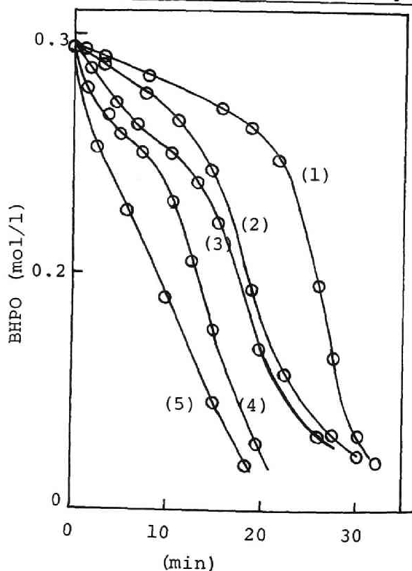
Fig. 3 Decomposition of BHPO catalyzed by \text{CuCl}_2 in pyridine at 35^\circ\text{C} \text{N}_2 atmosphere [\text{CuCl}_2] (\times 10^4 \text{ mol/l}) - (1) 5.0 (2) 10 (3) 20 (4) 40 (5) 80
