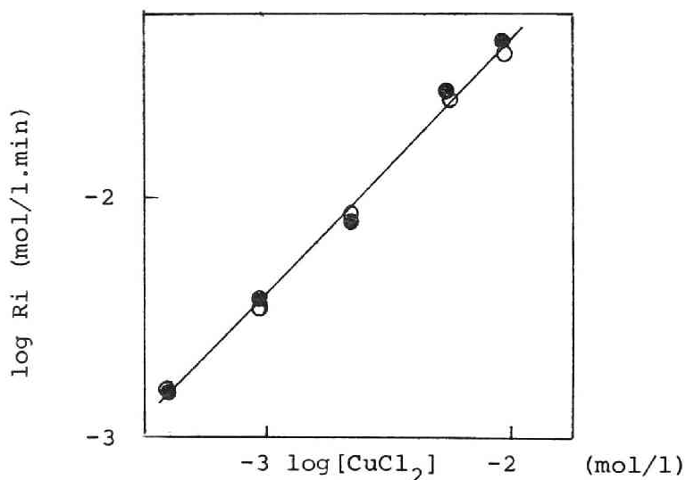
Fig. 8 Decomposition of BHPO catalyzed by \text{CuCl}_2 in pyridine [\text{BHPO}] = 0.192 \text{ mol/l} O under an atmospheric condition ● under a nitrogen atmosphere
