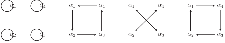
Figure 1: (\Omega, \Delta_i) (Form left, i = 1, i = 2, i = 3, i = 4 )
