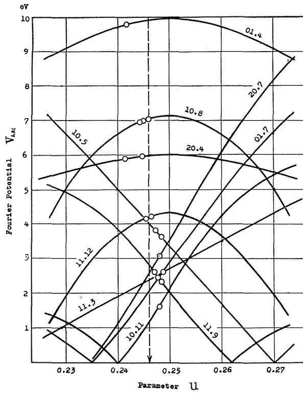
Fig. 5. Fourier potential versus parameter curves of \text{CdBr}_2 .
