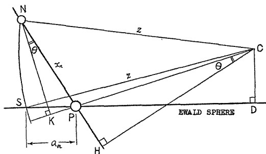
Fig. 7. Schematic illustration of the analysis of subsidiary maxima in elongated diffraction spots for an arbitrary rotation axis.
