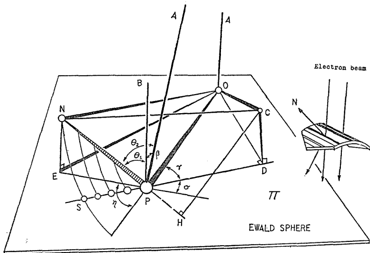
Fig. 6. Schematic illustration of the rotation of the reciprocal lattice for the arbitrarily warping crystal.
