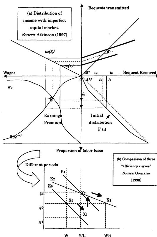
Fig. 1. Rising Earnings Dispersion Model
