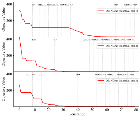
Fig. 14: Adaptive DR-NGnet optimization histories for three test cases, with gray lines indicating dimension expansion.
