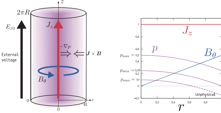
Fig.1 Z-pinch equilibrium in cylindrical geometry
