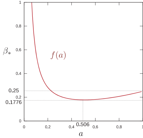
Fig.5 Plot of \beta_* = f(a) .
