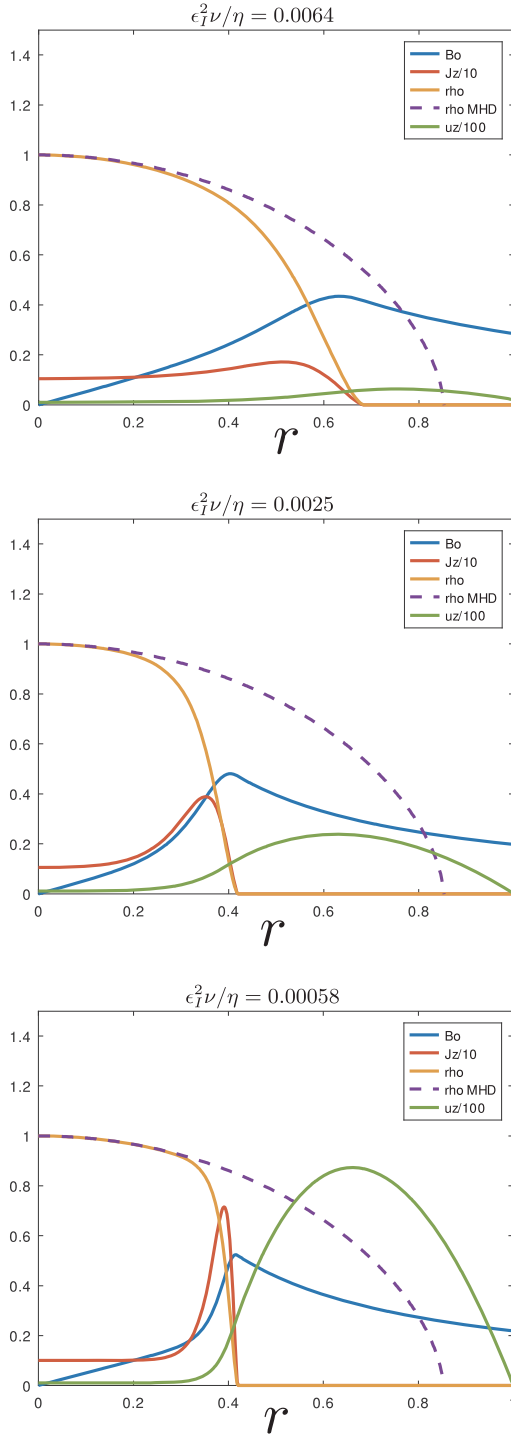
Fig.4 XMHD solution with the viscosity (29) where \gamma = 5/3 , \beta = 0.018 .
