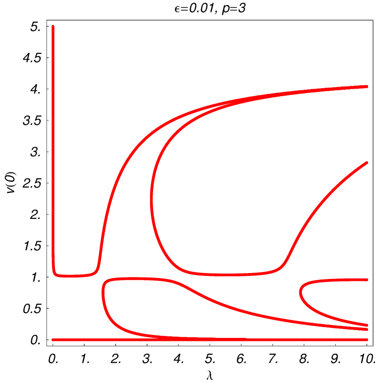
Fig 1: The diagram of (1) with n = 3 and p = 3 .
