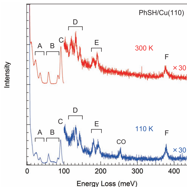
FIG. 5. EEL spectra recorded for \text{C}_6\text{H}_5\text{SH}/\text{Cu}(110) at 300 K (top) and 110 K (bottom). Either spectrum shows no S–H stretch peak at \sim 300 meV, indicating that thiophenol is dehydrogenated to thiophenoxo species even at 110 K. The peak assignment is summarized in Table II.
