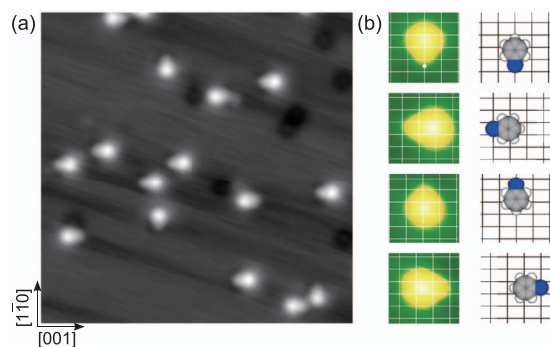
FIG. 4. (a) A typical STM image of Cu(110) exposed to thiophenol at 78 K ( V = 50 mV and I = 5 nA). Thiophenol is dehydrogenated to thiophenoxo ( \text{C}_6\text{H}_5\text{S} ) group which is oriented along either [1\bar{1}0] or [001] direction. (b) STM images of thiophenoxo groups in different orientations ( V = 50 mV and I = 1 nA), and their schematic illustrations. Sulfur atom is adsorbed on the short-bridge site with the phenyl ring nearly parallel to the surface. The image size is 140 \times 140 \text{ \AA}^2 and 14 \times 14 \text{ \AA}^2 for (a) and (b), respectively.
