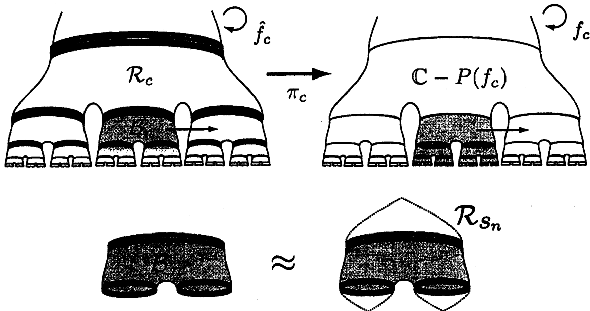
Figure 2: A caricature of blocks in \mathcal{R}_c .
