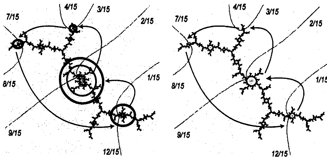
Figure 1: Any simple renormalization determines a unique superattracting parameter.
