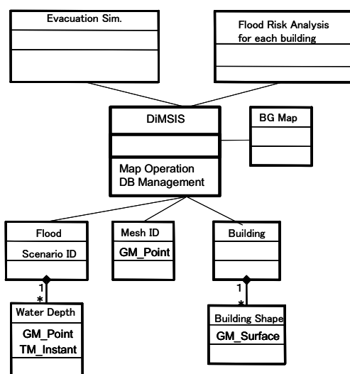
Fig. 3 UML Diagram of Developed System
