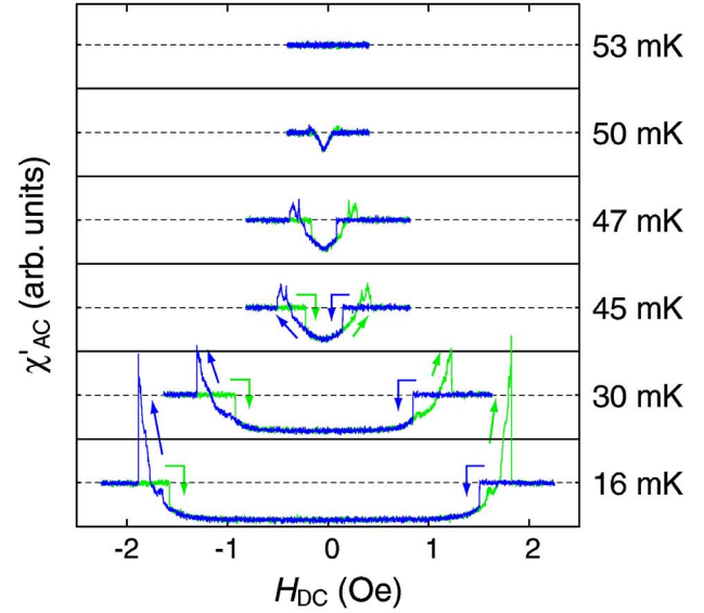
FIG. 2. (Color online) ac susceptibility of \text{Ag}_5\text{Pb}_2\text{O}_6 . (a) The result of a temperature sweep with a sweep rate of 0.2 mK/min. The residual field H_{\text{res}} has been compensated in this sweep, yielding T_{c0} = 52.4 mK. (b) The results of field sweeps at several temperatures with a sweep rate of 24–47 mOe/min. From the slight asymmetry of the data, the residual field is estimated as H_{\text{res}} = 0.040 Oe. The double peaks seen in 45 and 47 mK do not seem to be intrinsic, since they are not reproducible with other crystals.
