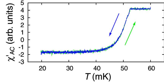
(b) \text{Ag}_5\text{Pb}_2\text{O}_6 , H_{\text{DC}} \parallel c
