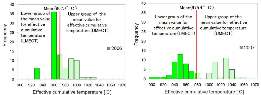
(a) effective cumulative temperature in 2006 (b) effective cumulative temperature in 2007 Fig. 7. Histograms of effective cumulative temperature for each field in 2006 and 2007
