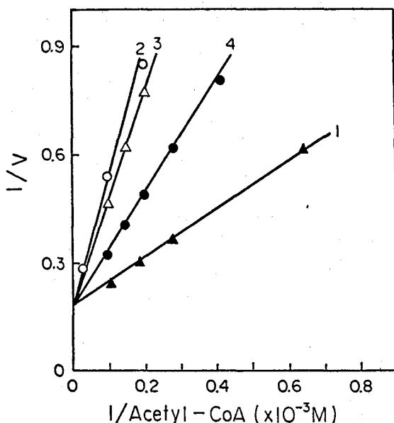
Fig. 10. Inhibition of S -( \beta -aminoethyl)-L-cysteine \omega - N -acetyltransferase by propionyl-CoA, butyryl-CoA and benzoyl-CoA.
