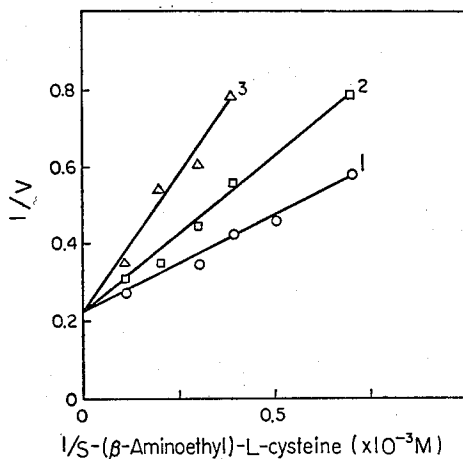
Fig. 11. Inhibition of S -( \beta -aminoethyl)-L-cysteine \omega - N -acetyltransferase by S -( \beta -aminoethyl)- \alpha - N -acetyl-L-cysteine and S -( \beta -aminoethyl)-mercaptopyruvate.
