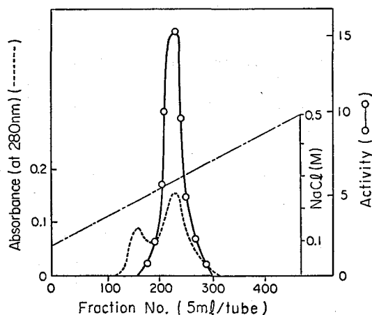
Fig. 4. Second DEAE-cellulose column chromatography.
