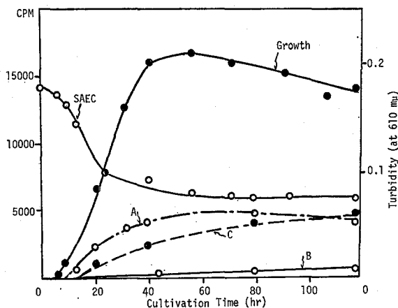
Fig. 2. Incorporation of the radioactivity into the products from S -( \beta -aminoethyl)-L-[ 35 S]-cysteine during bacterial growth.
