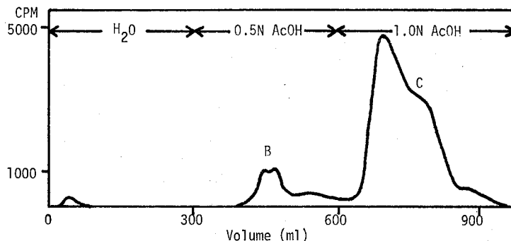
Fig. 4. Chromatography of Fraction I on Dowex-1x8.
