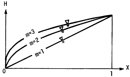
Fig. 5 Profiles of water surfaces in steady states for m=1, 2 and 3
