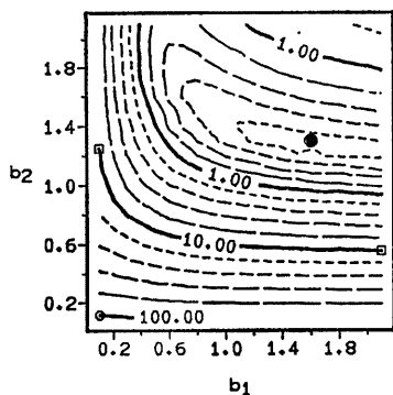
Fig. 3 Isopleth of the sums of simulation errors for various sets of b_1, b_2 . The number of reservoirs is 2.
