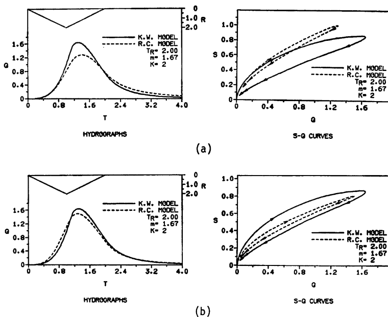
Fig. 2 Simulation of kinematic wave flows by reservoir cascade models (a) with b_1=1 and (b) with b_1 given by eq. (3.4)
