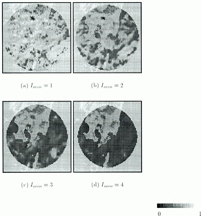
fig 7 Distribution of temporal continuity of growth-decay rate
