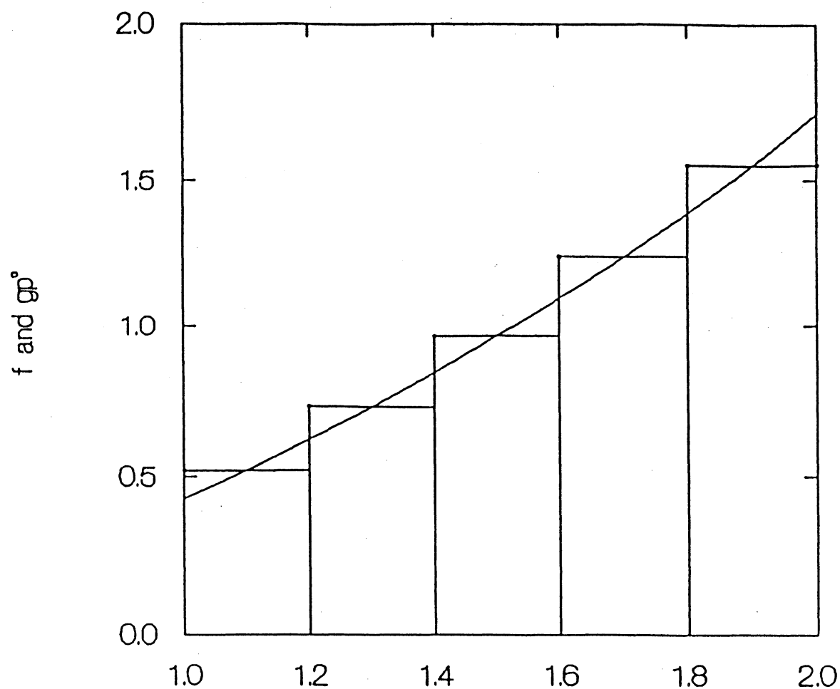
Figure 2: A quadratic underlying density and its theoretical histogram.
