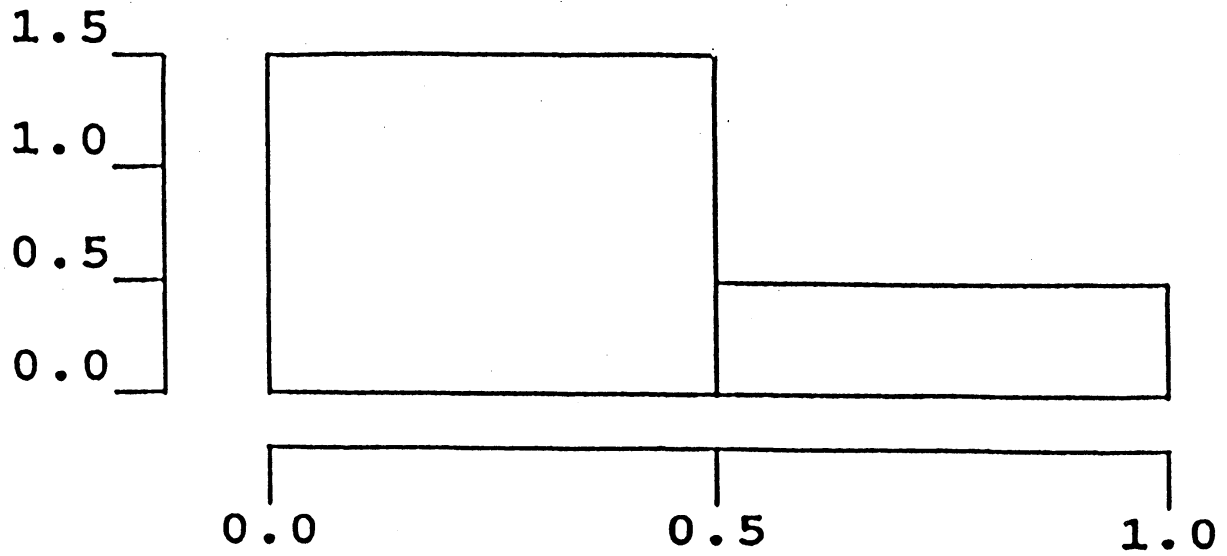
Figure 1: A finite mixture of uniforms. The theoretical histogram coincides with the underlying density.
