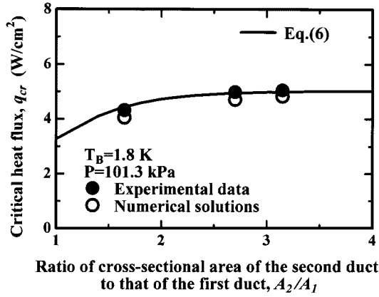
Fig. 2. Critical heat flux versus ratio of cross-sectional area of the second duct to that first duct.
