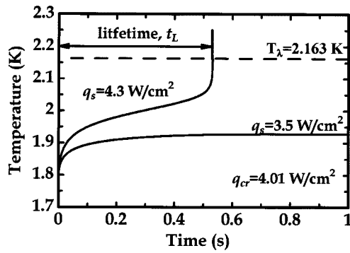
Fig. 6. Typical time trace of liquid temperature adjacent to the heated surface, T_h , for various step heat inputs, q_s .
