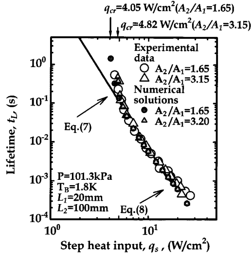
Fig. 4. Lifetime versus step heat flux.
