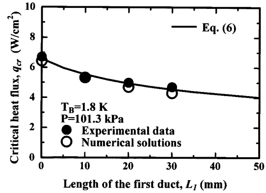
Fig. 3. Critical heat flux versus length of the first duct.
