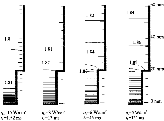
Fig. 7. Temperature distribution in a duct with A_2/A_1 = 1.65 for various step heat fluxes.
