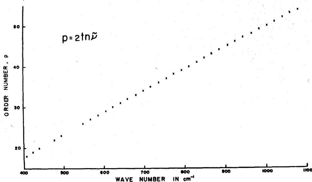
Fig. 6 Relation between Order Number and Position of Transmission Interference Fringes
