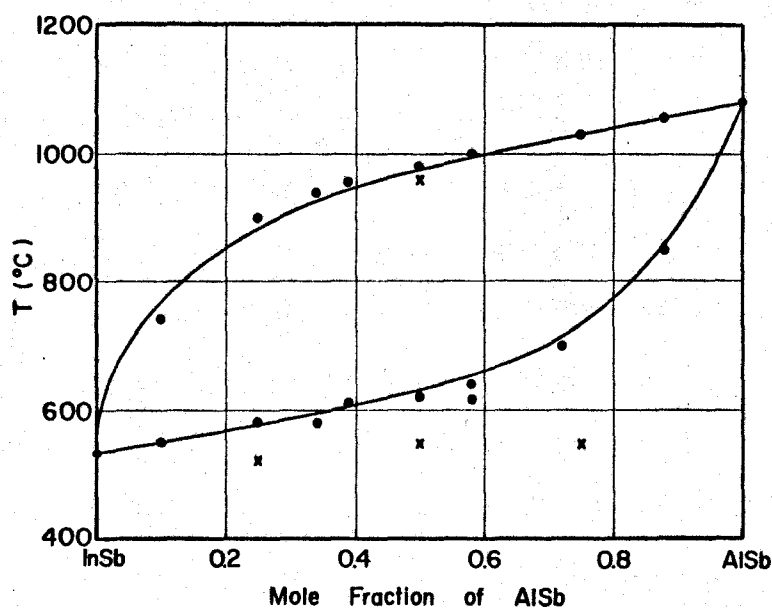
Fig. 11 InSb-AlSb phase diagram Experimental values given by D. Effer 37) and solid lines calculated.
