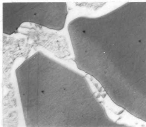
Photo. 1 Microphotograph of GaSb-50 mol% GaAs alloy
