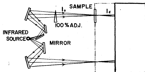
Fig. 1 Experimental arrangement
