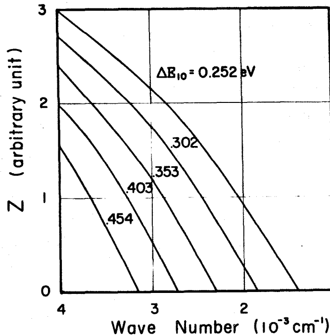
Fig. 23 Wave number dependence of theoretical Z parameter
