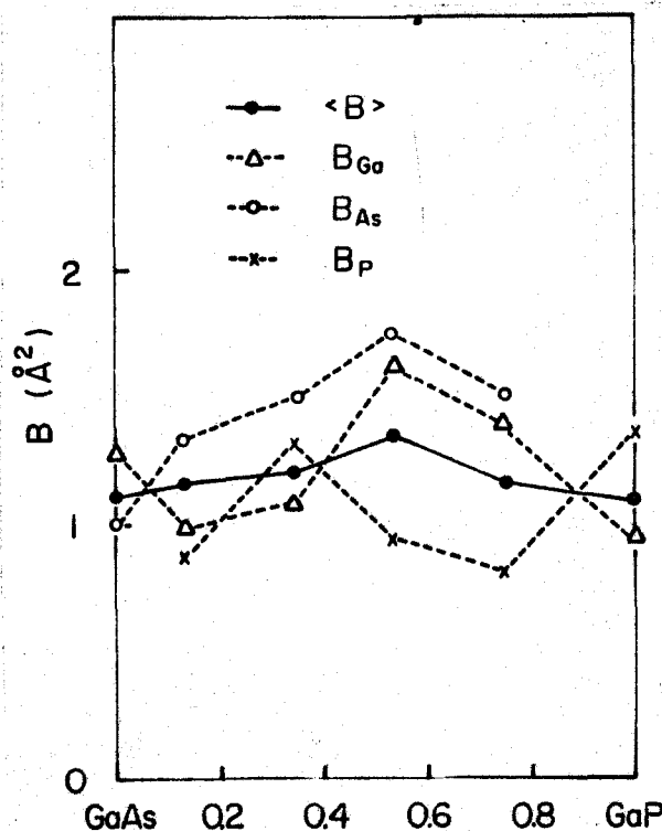
Fig. 3 Temperature factors in GaAs, GaP and their alloys
