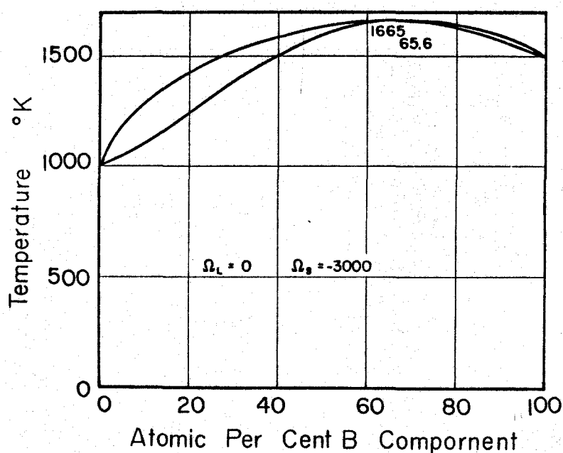
Fig. 16 Calculating binary phase diagrams under the approximation of regular solution
