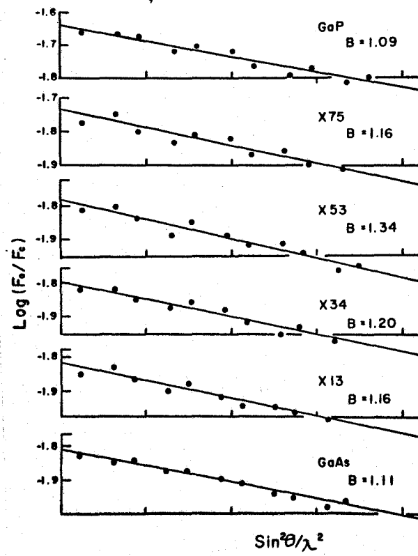
Fig. 1 \log(F_{\text{obs}}/F_{\text{cal}}) v.s. \sin^2\theta / \lambda^2
