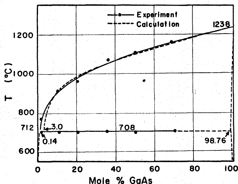
Fig. 5 GaAs-GaSb phase diagram
