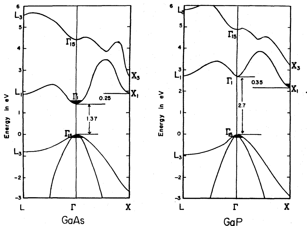
Fig. 8 Energy band structures of GaAs and GaP
