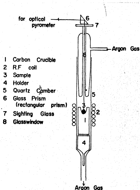
Fig. 1 The apparatus for measuring melting points
