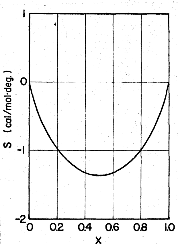
Fig. 13 Entropy of mixing
