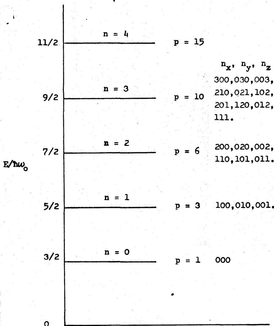
Fig. 32 Energy levels, degrees of degeneracy, and quantum numbers for the three dimensional isotropic harmonic oscillator
