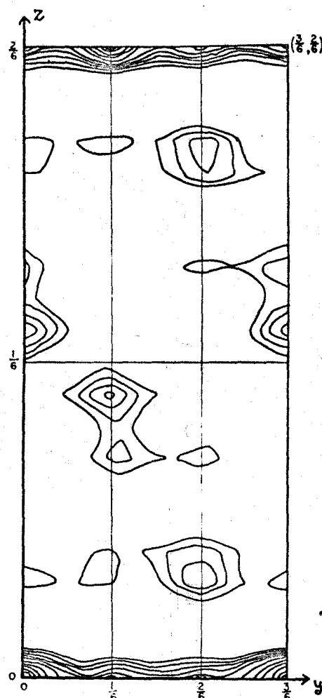
\beta Phase b_1 = 6.97\text{\AA} c = 29.41\text{\AA}
