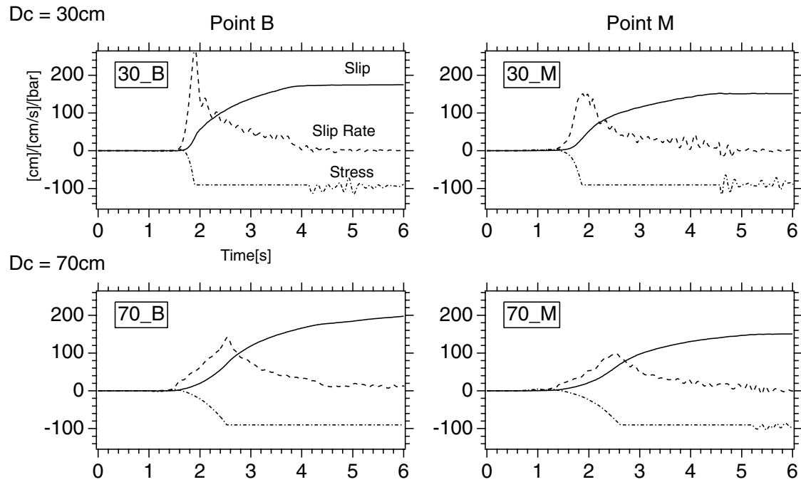
Figure 10. Time histories of stress, slip, and slip velocity at two selected points B(b) and M(m), calculated from the dynamic rupture for prescribed values of D_c = 30\text{ cm} and D_c = 70\text{ cm} .
