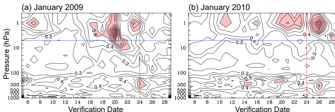
Fig. 8. (a) Same as Fig. 5, except for the growth rate ( \text{day}^{-1} ) of the most unstable mode computed for the basic flow consisting of the T21 truncated stream function at each pressure level (the ordinate) of the 4-day ensemble mean forecast. The contour interval is 0.1 \text{ day}^{-1} , and regions where the growth rate is larger than 0.6 ( 1.0 ) \text{day}^{-1} are lightly (heavily) shaded in red. (b) Same as (a), except for January 2010.
