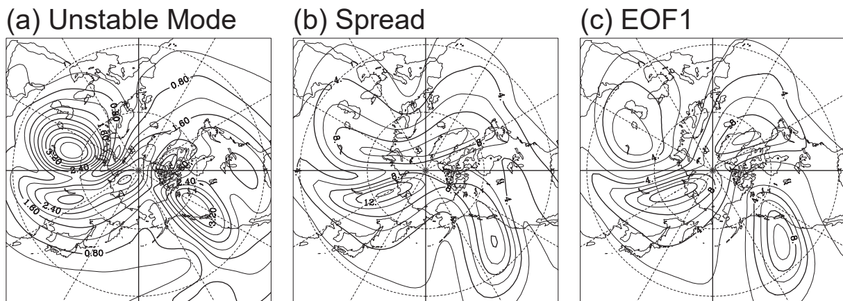
Fig. A1. (a) Horizontal distribution for the square root of the variance of the stream function associated with the phase variation of the most unstable mode on day -4 (middle panel of Fig. 9c). (b) Same as (a), except for the square root of ensemble spread of the predicted stream function on day -4 , computed using the 4-day ensemble forecast starting from day -7 . (c) Same as (b), except for the absolute value of the regressed stream function anomaly onto PC1 of the ensemble spread on day -4 . PC1 is the corresponding principal component score to the 1st EOF shown in Fig. 6c. The contour interval is 2 \times 10^6 \text{ m}^2 \text{ s}^{-1} in (b) and (c). The magnitude in (a) is arbitrary.
