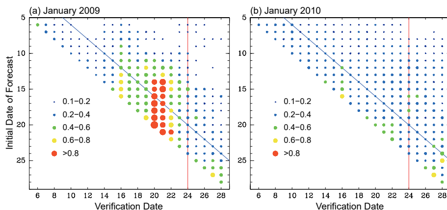
Fig. 7. (a) Growth rate ( \text{day}^{-1} ) of the most unstable mode computed for the basic flow consisting of the T21 truncated 5-hPa stream function of the ensemble mean field on each prediction date (the abscissa) of the forecast starting from 6 to 28 January (the ordinate). The radius of the filled circle is proportional to the growth rate, and its color also indicates the range of the growth rate as shown in the legend. The red vertical line represents day 0 (24 January), and the blue slanting line indicates 4-day forecasts. (b) Same as (a), except for January 2010.
