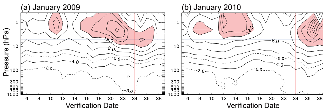
Fig. 5. (a) Amplification rate of the rms ensemble spread during the 4-day forecast at each pressure level (the ordinate) for each verification date (the abscissa) in January 2009. Spreads were evaluated based on geopotential height fields north of 30°N. Regions with an amplification rate larger than 12.0 are shaded in red. The red vertical line denotes day 0 (24 January), and the blue horizontal line represents 5 hPa. (b) Same as (a), except for January 2010.
