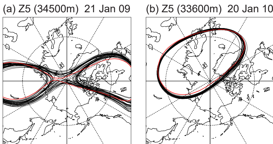
Fig. 3. Limited contour analysis of polar vortex, showing contours at a prescribed 5-hPa height of 34500 m on 21 January 2009 (a) and 33600 m on 20 January 2010 (b). Thick red curves show the analysis (ERA-Interim). The corresponding 4-day ensemble forecasts are shown by thin black curves.
