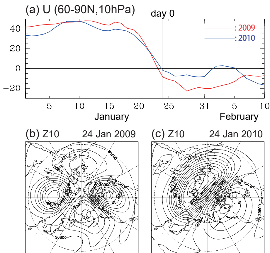
Fig. 1. (a) Time evolution of the zonal-mean zonal wind averaged poleward of 60^\circ\text{N} at 10 hPa ( \text{m s}^{-1} ) during the winter seasons of 2009 (red line) and 2010 (blue line) for the analysis (ERA-Interim). (b) Horizontal distribution of 10-hPa geopotential height (m) on 24 January 2009 for the analysis. The contour interval is 200 m. (c) Same as (b), except for 24 January 2010.
