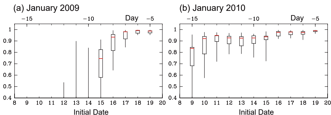
Fig. 2. Spatial anomaly correlation coefficient (ACC) for the predicted 10-hPa geopotential height on day 0 (24 January) for ensemble forecasts starting from 9 (day -15) to 19 (day -5) January (the ordinate). The spatial ACC is evaluated poleward of 40^\circ\text{N} . The whiskers indicate the full range of ACCs for 25 ensemble members, and the boxes show the range between the 6th value from the largest (24 %) and the 7th value from the smallest (76 %) ACCs. Short horizontal red lines indicate ACCs for the ensemble mean forecasts.
