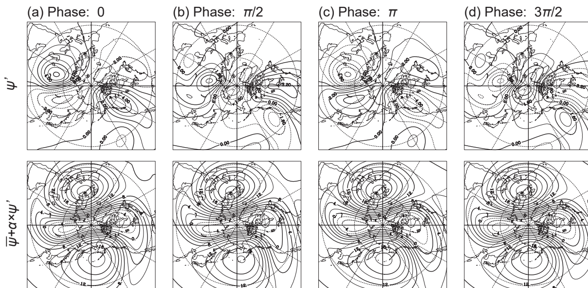
Fig. 10. (Top) The stream function field of the most unstable mode (middle panel of Fig. 9c) on day -4 at each 1/4 phase of period 2\pi : (a) phase 0 (initial), (b) phase \pi/2 , (c) phase \pi , and (d) phase 3\pi/2 . (Bottom) Same as the top panels, except for the composited stream function field ( 10^7 \text{ m}^2 \text{ s}^{-1} ) of the basic flow (top panel of Fig. 9c) and the most unstable mode at each 1/4 phase with amplitude \alpha . The amplitude \alpha is specified so that the square root of the variance of the stream function of the unstable mode at the initial phase (a) is 7.24 % of that of the basic flow. The variance is evaluated in the region north of 30^\circ\text{N} .
