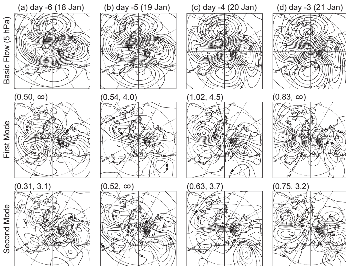
Fig. 9. (Top) Horizontal structure of the basic flow given by the T21 truncated 5-hPa stream function field ( 10^7 \text{ m}^2 \text{ s}^{-1} ) of the ensemble mean prediction on day -6 (a), day -5 (b), day -4 (c), and day -3 (d) for the 4-day forecasts during January 2009. (Middle and bottom) Stream function fields for the first and second unstable modes computed for the basic flow. The first and second numbers in parentheses at the top of each panel indicate the growth rate ( \text{day}^{-1} ) and the period (day) of the unstable mode, respectively. Stationary modes with zero imaginary component of eigenvalues are designated by the period of infinity ( \infty ).
