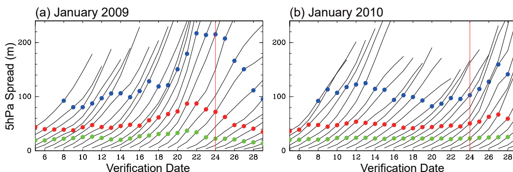
Fig. 4. Time evolution of the rms ensemble spread (m) during the 10-day forecast based on the 5-hPa geopotential height field north of 30°N. See text for the detailed definition of the rms ensemble spread. (a) January 2009. (b) January 2010. Green, red, and blue solid circles indicate 2-, 4-, and 7-day forecasts, respectively.
