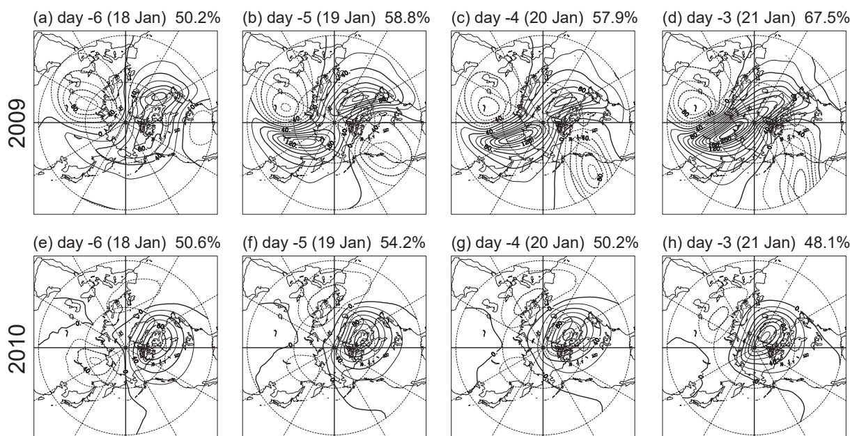
Fig. 6. The 1st EOFs of the difference field of each ensemble member from the ensemble mean prediction of the 5-hPa geopotential height north of 30^{\circ}\text{N} (m) during the onset of the 2009 SSW (top panels) and 2010 SSW (bottom panels) on day -6 (a, e), day -5 (b, f), day -4 (c, g), and day -3 (d, h), computed using 4-day forecasts. Contours are scaled to represent anomalies in meters when the PC is equal to one standard deviation; the contour interval is 20 m. Percentage variances associated with the 1st EOFs are shown in the upper right of each panel.
