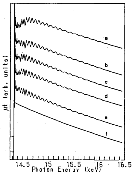
Fig. 3. The simulation of X-ray absorption spectra on Kr including multielectron transition process.
