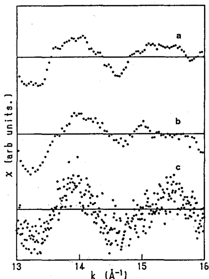
Fig. 2. XAFS of Zn foil with and without the low-pass filter.
