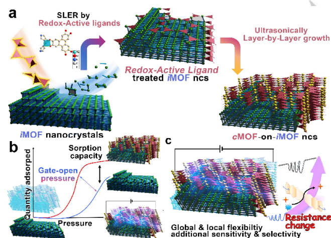
Figure 1. Design of the heterostructures and structure-function relationships. (a) Schematic of the ultrasonically LbL LPE preparation of cMOF-on-/iMOF heterostructured nanocrystals (ncs), and the corresponding (b) responsive gas/vapor adsorption with/without electrical control, and (c) electrically-transduced soft porosity related chemiresistive gas/vapor sensing.
