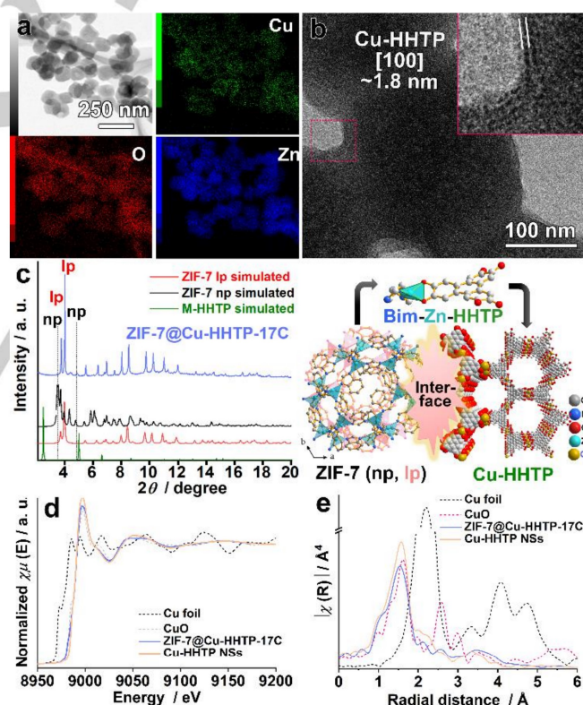
Figure 2. TEM, PXRD, XANES and EXAFS of ZIF-7@Cu-HHTP-17C ncs. (a) The TEM image of ZIF-7@Cu-HHTP-17C ncs followed by the corresponding EDS mapping images of Cu, O, and Zn. (b) Cu-HHTP sheath of ZIF-7@Cu-HHTP-17C showing (100) face (the inset is the enlarged image of the red zone), (c) the synchrotron PXRD patterns of ZIF-7@Cu-HHTP-17C compared with simulated ZIF-7, Cu-HHTP and possible hybrid bonds. Data were collected at beamline 02B2 in SPring 8, Japan ( \lambda=0.79962 Å), (d) Cu K-edge XANES spectra. Data were collected at beamline BL11S2 in the Aichi Synchrotron Radiation Center, Japan; and (e) Fourier transform EXAFS of Cu foil, CuO, Cu-HHTP, ZIF-7@Cu-HHTP-xC (x=10, 17), and ZIF-7@Cu-HITP-5C.
