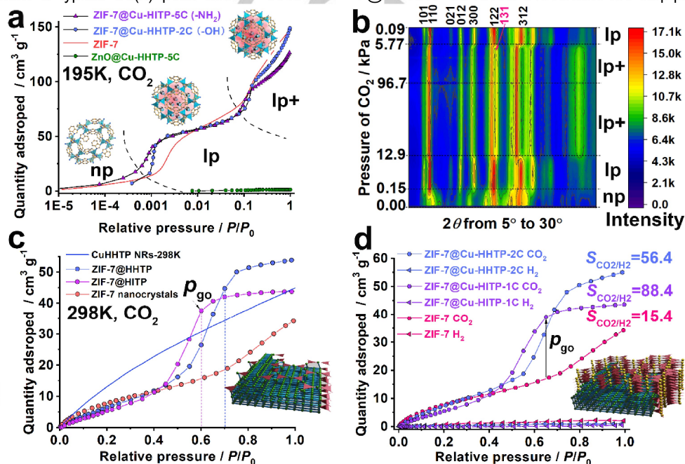
Figure 3. The modulated soft porosity without electrical control. (a) CO 2 sorption isotherm at 195 K of ZIF-7@cMOFs compared with bare ZIF-7 ncs; (b) The contour plot for the in situ PXRD patterns of ZIF-7@Cu-HITP-5C upon exposure to CO 2 with varying pressure; (c) CO 2 sorption isotherm of Cu-HHTP NRs, ZIF-7 ncs, and ligand treated ZIF-7 ncs (ligand=HITP, HHTP) at 298 K; (d) CO 2 /H 2 selectivity comparison of ZIF-7 and ZIF-7@cMOFs at 298 K.
